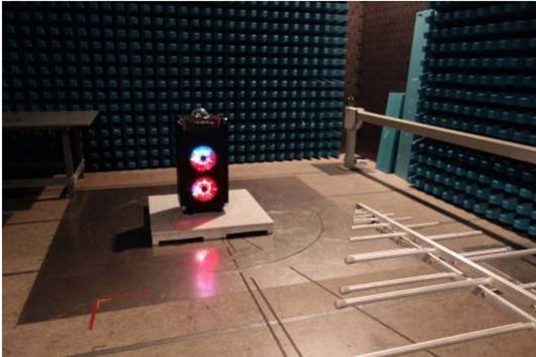
Re (30M-1GHz)
