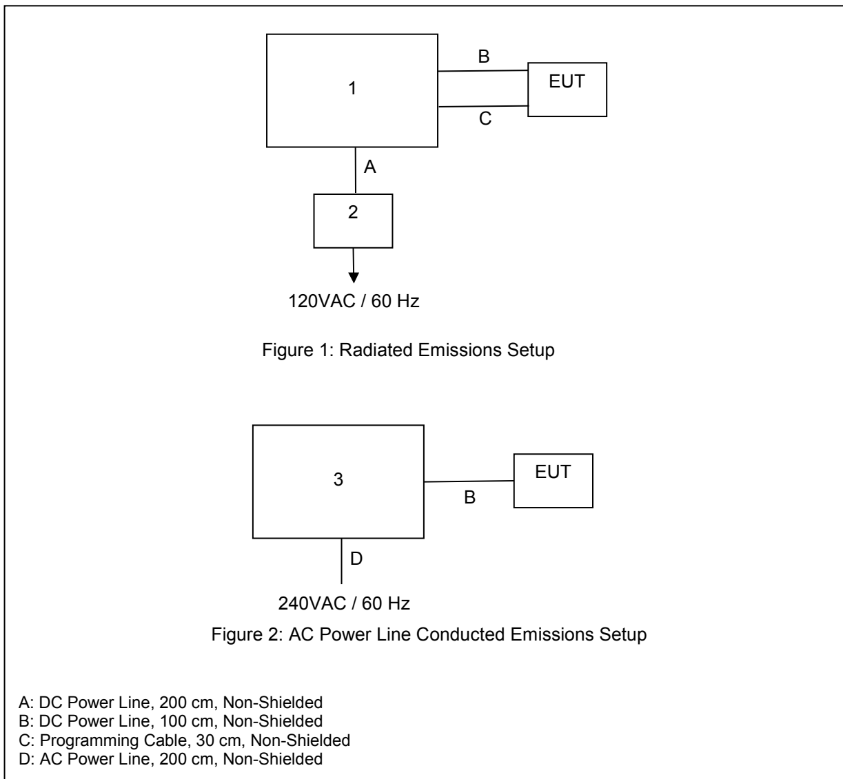
Figure 6-1: Test Setup Block Diagram
