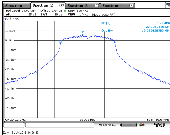
Figure 7.3.2-10: 99% OBW – 802.11g – 2412MHz
