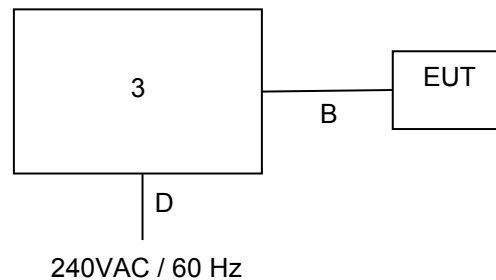
Figure 2: AC Power Line Conducted Emissions Setup
