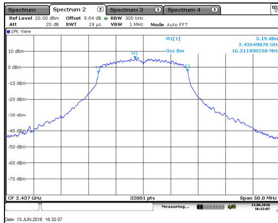
Figure 7.3.2-11: 99% OBW – 802.11g – 2437MHz
