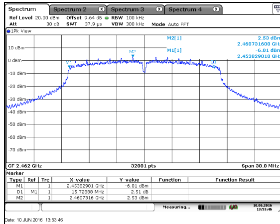
Figure 7.3.2-9: 6dB BW – 802.11g – 2462MHz
