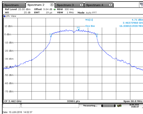
Figure 7.3.2-12: 99% OBW – 802.11g – 2462MHz
