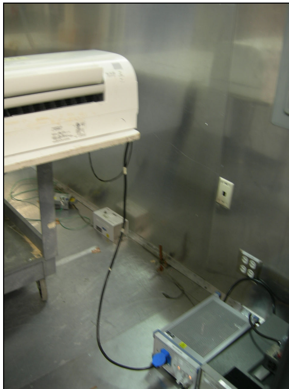
Figure 8: Conducted Emissions
