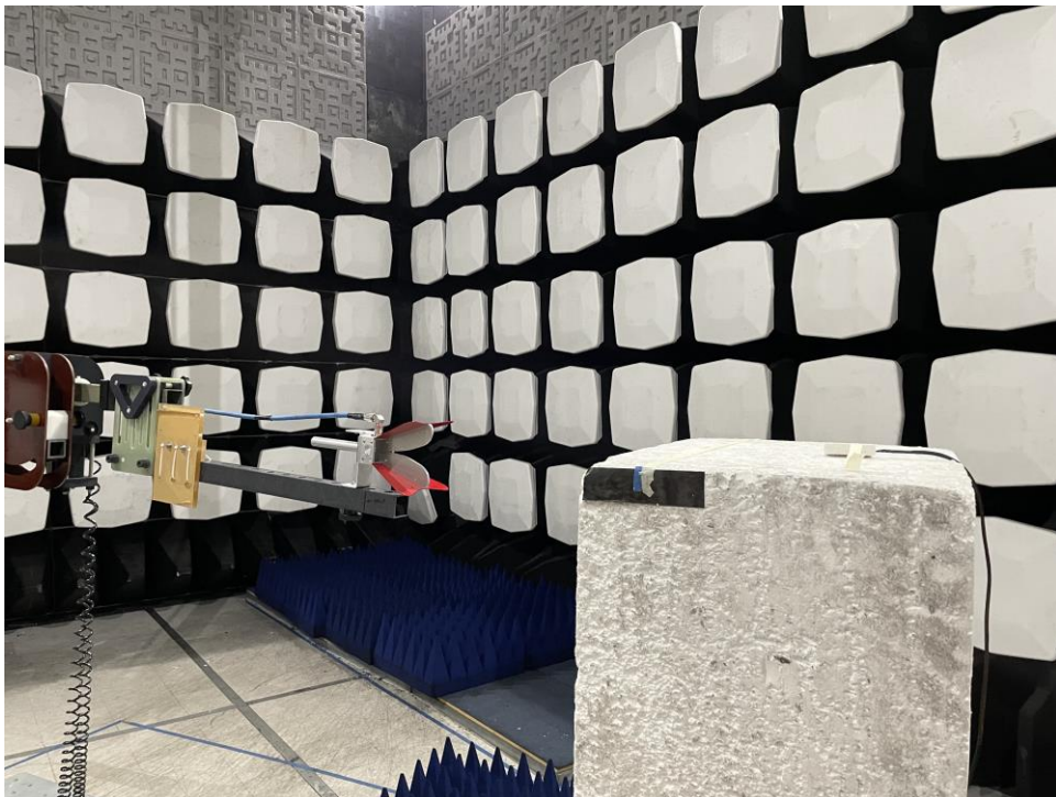
Figure 4 – Test Set up - Radiated Emissions <18 GHz
