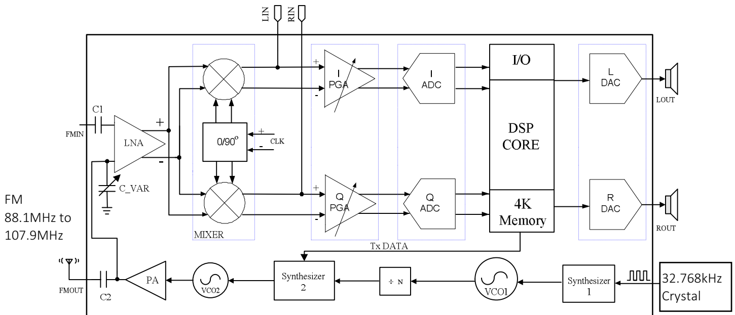
Figure 3-1. RDA5820 FM Transceiver Block Diagram
