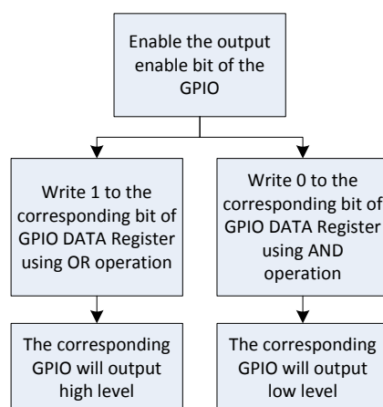
Figure 11-4 GPIO Output Configuration
