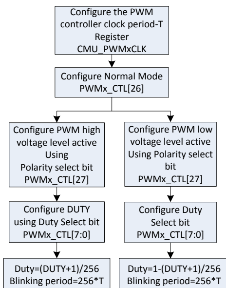
Figure 13-8 PWM Configuration
