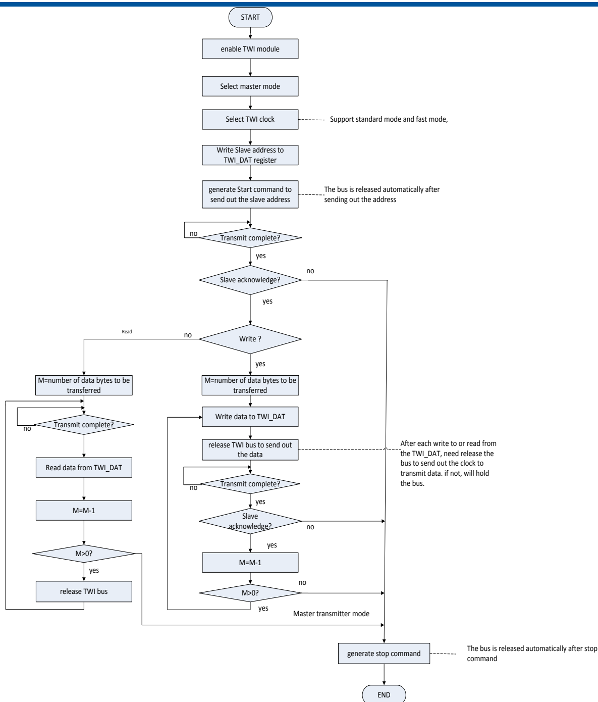
Figure 10-1 TWI Master Mode Operation Flow
