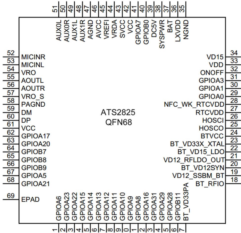
Figure 1-2 ATS2825 (QFN68) Pin Assignment
