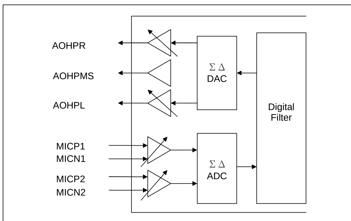
Figure 6.10 Audio Codec
