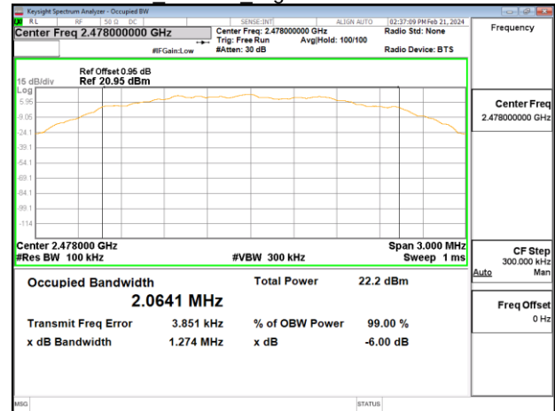
OBW BLE 2M HighCH38-2478MHz
