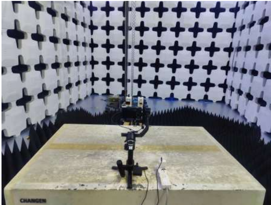
3. Radiated Emissions (Part 15B Normal Working, 18GHz-26.5GHz)
