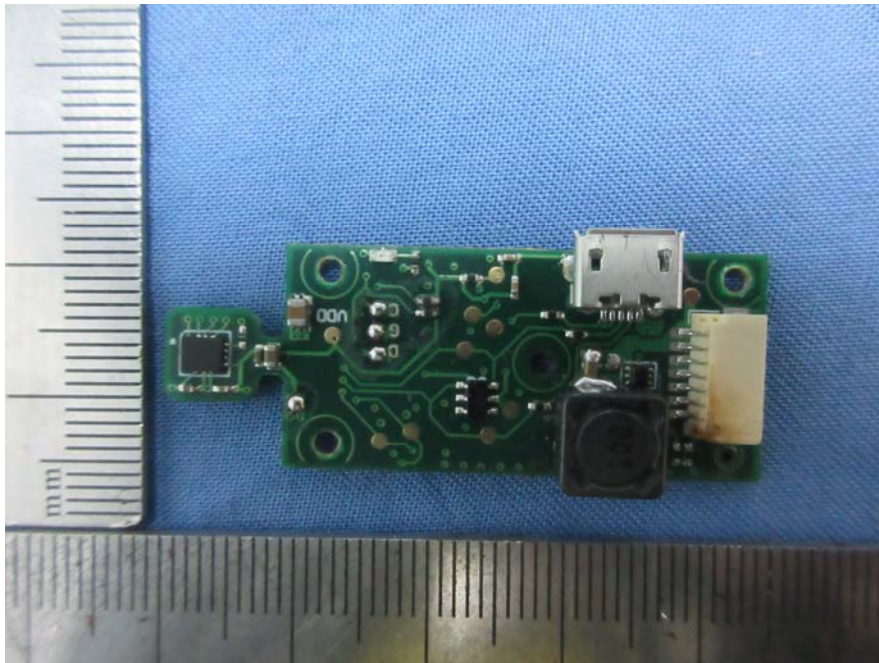
EUT- PCB Board Top View (Micro-USB output)
