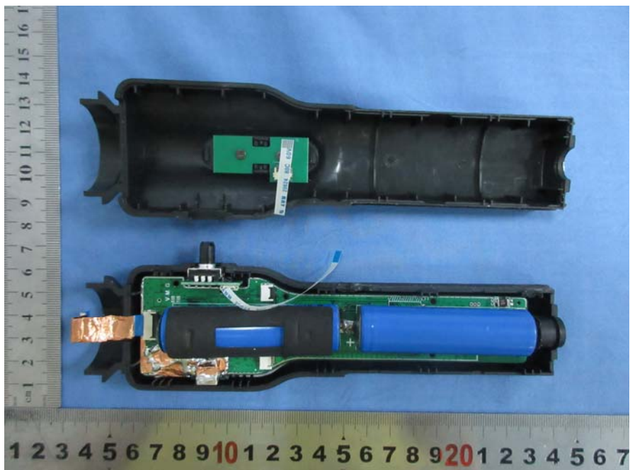
EUT – Uncovered 4 View
