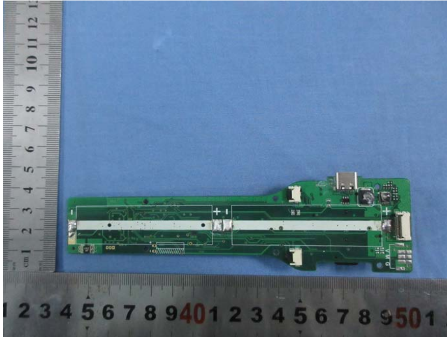
EUT – PCB Board Bottom View (Main control)
