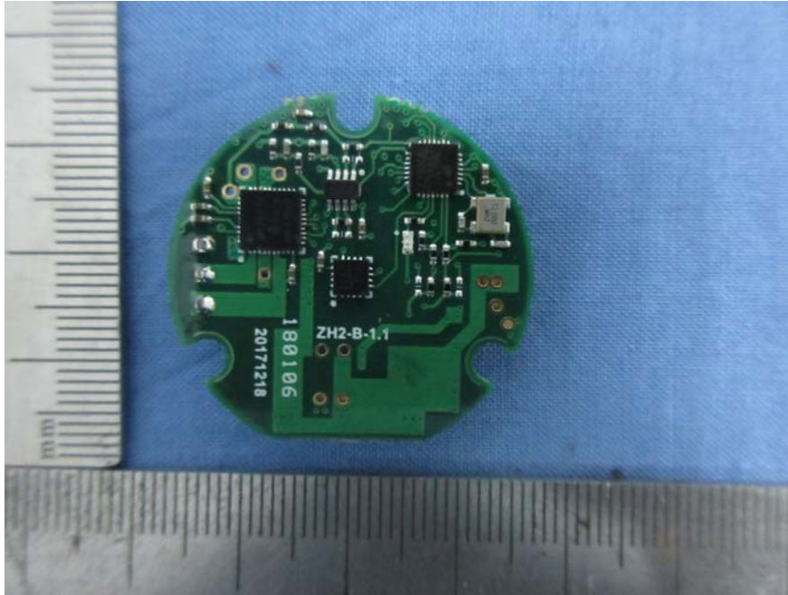
EUT – PCB Board Bottom View (Stabilizer bar axis 2)
