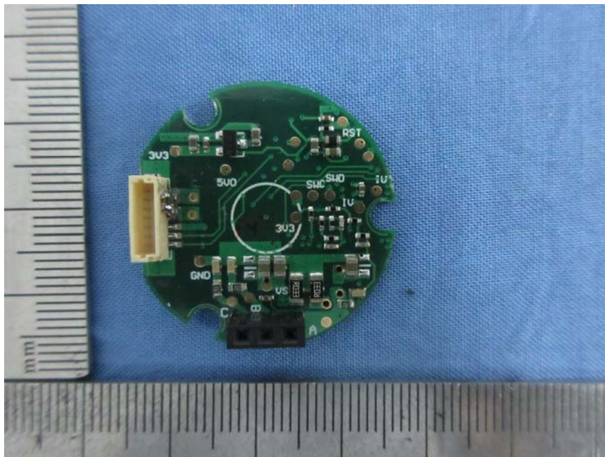
EUT – PCB Board Top View (Stabilizer bar axis 1)
