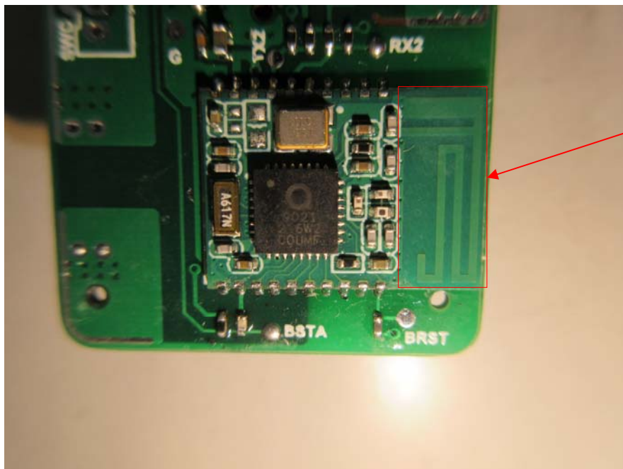
EUT – Blue Chip and Antenna View
