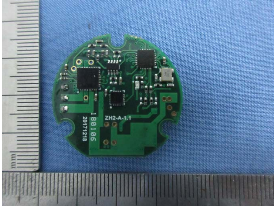
EUT – PCB Board Bottom View (Stabilizer bar axis 3)
