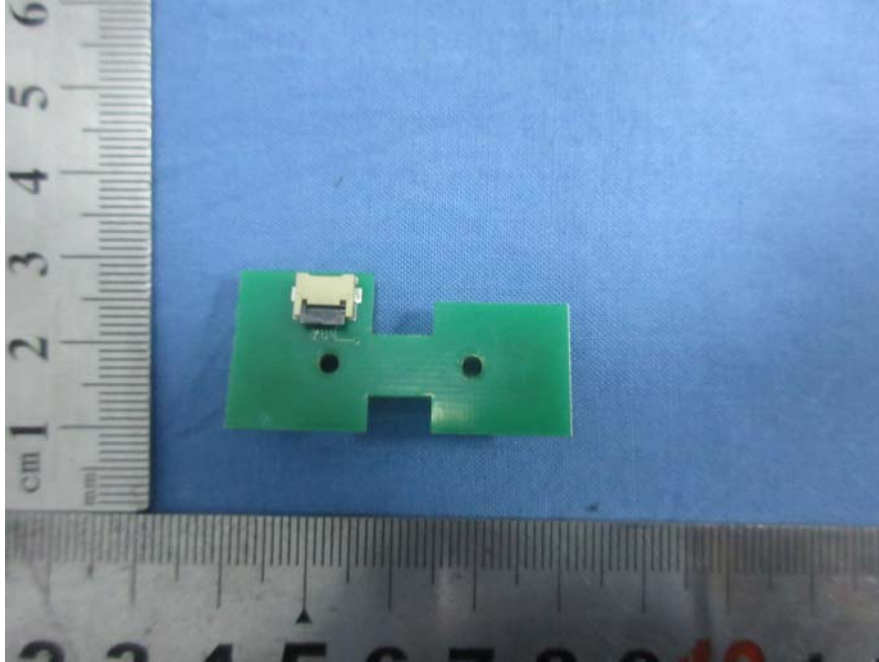
EUT – PCB Board Bottom View (Following button)
