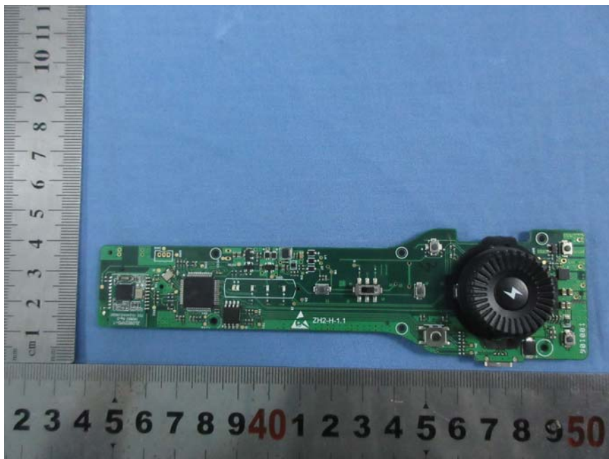
EUT – PCB Board Top View (Main control)
