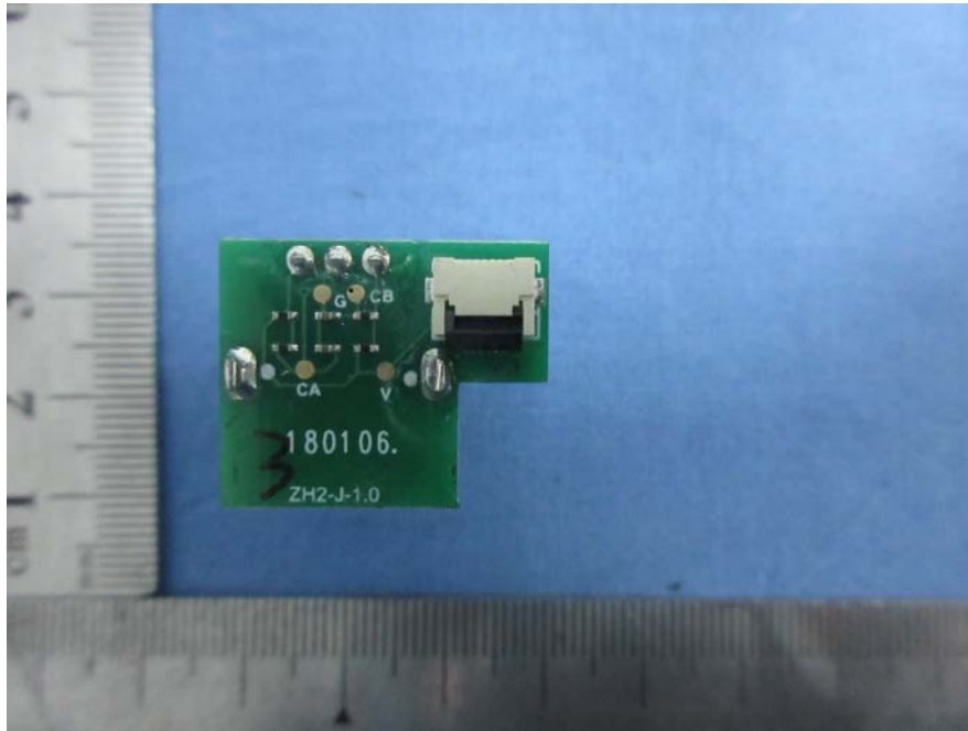
EUT – PCB Board Bottom View (Zoom button)
