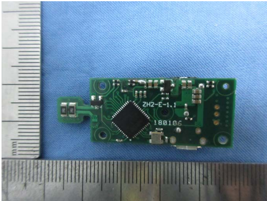
EUT- PCB Board Bottom View (Micro-USB output)
