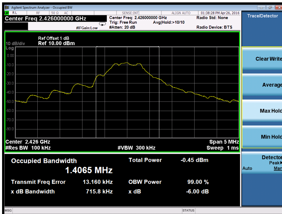
Figure 2: 6dB Bandwidth, 2426MHz
