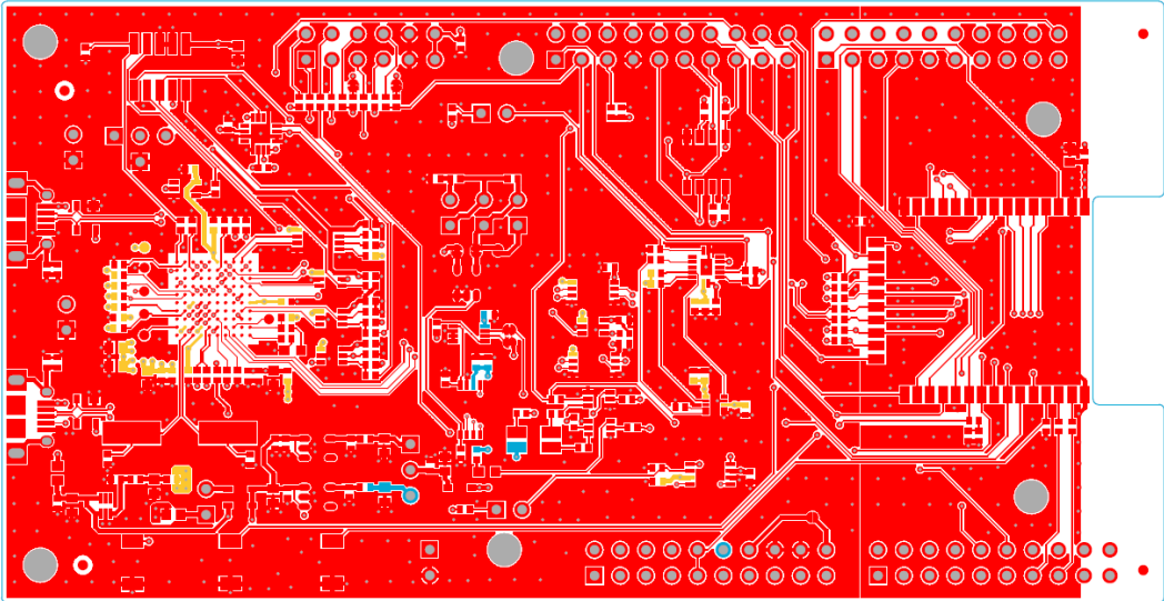
Figure 22 Top Etch
