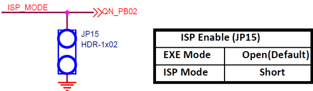
Figure 7 Chip mode jumper
