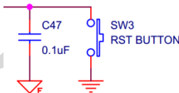
Figure 6 Reset button
