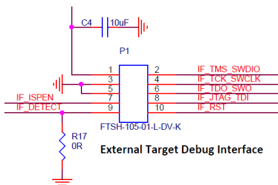
Figure 8 JTAG interface
