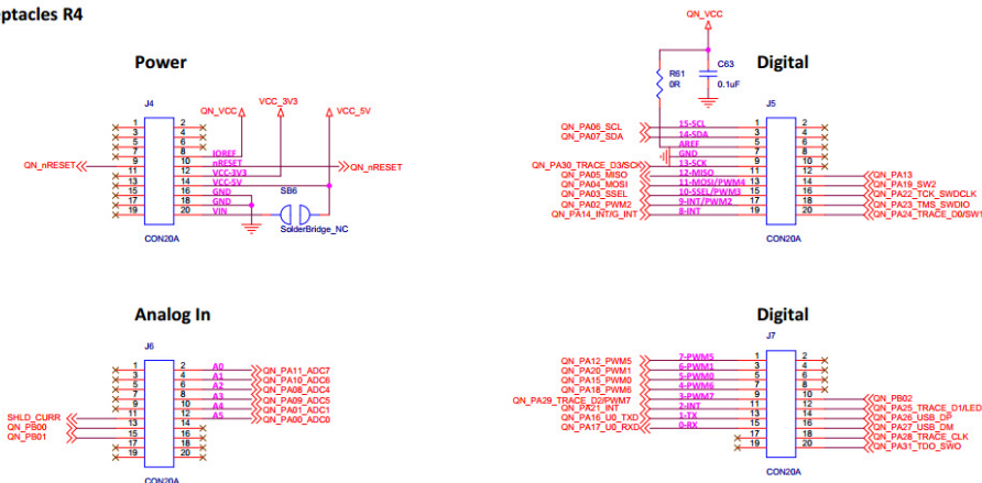
Figure 5 QN908x DK board GPIO and Arduino interface
