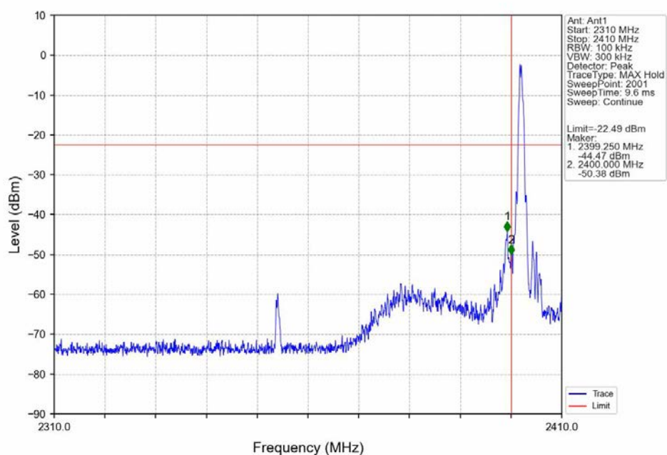
2.4G_LCH_2402MHz_Ant1_NTNV
