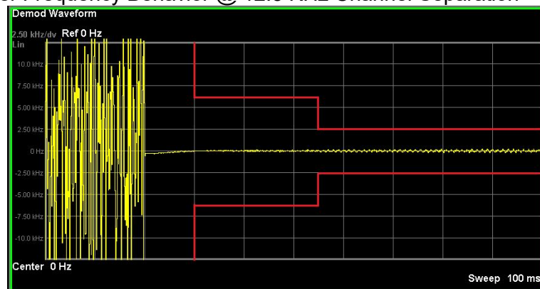
Transmitter Frequency Behavior @ 12.5 KHz Channel Separation-----Off – On
