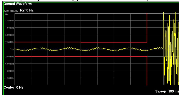
Transmitter Frequency Behavior @ 12.5 KHz Channel Separation-----On – Off
