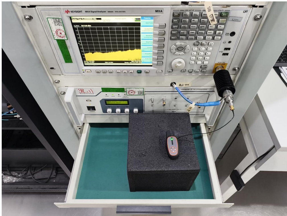
Test Setup Photo(s) of RF Measurement Fig.3
