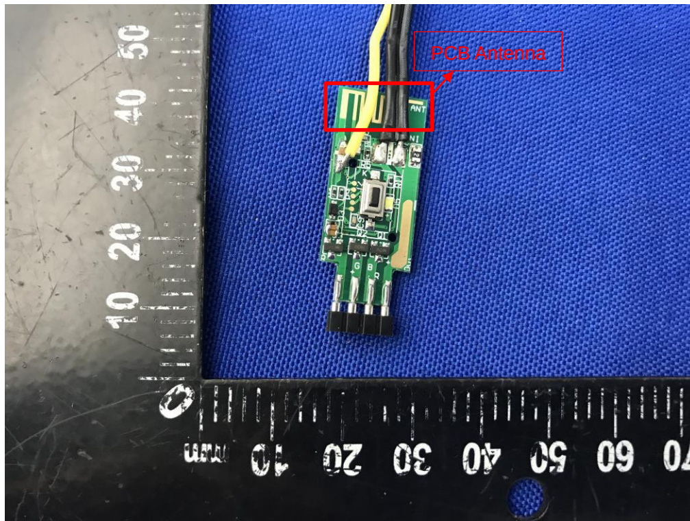
MAIN BOARD TOP VIEW (XK-MINI-TURN-KIT)
