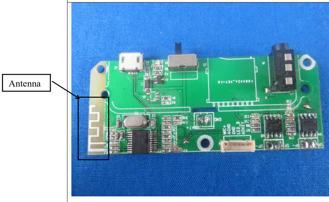
6. Figure PCB of the EUT-Front View
