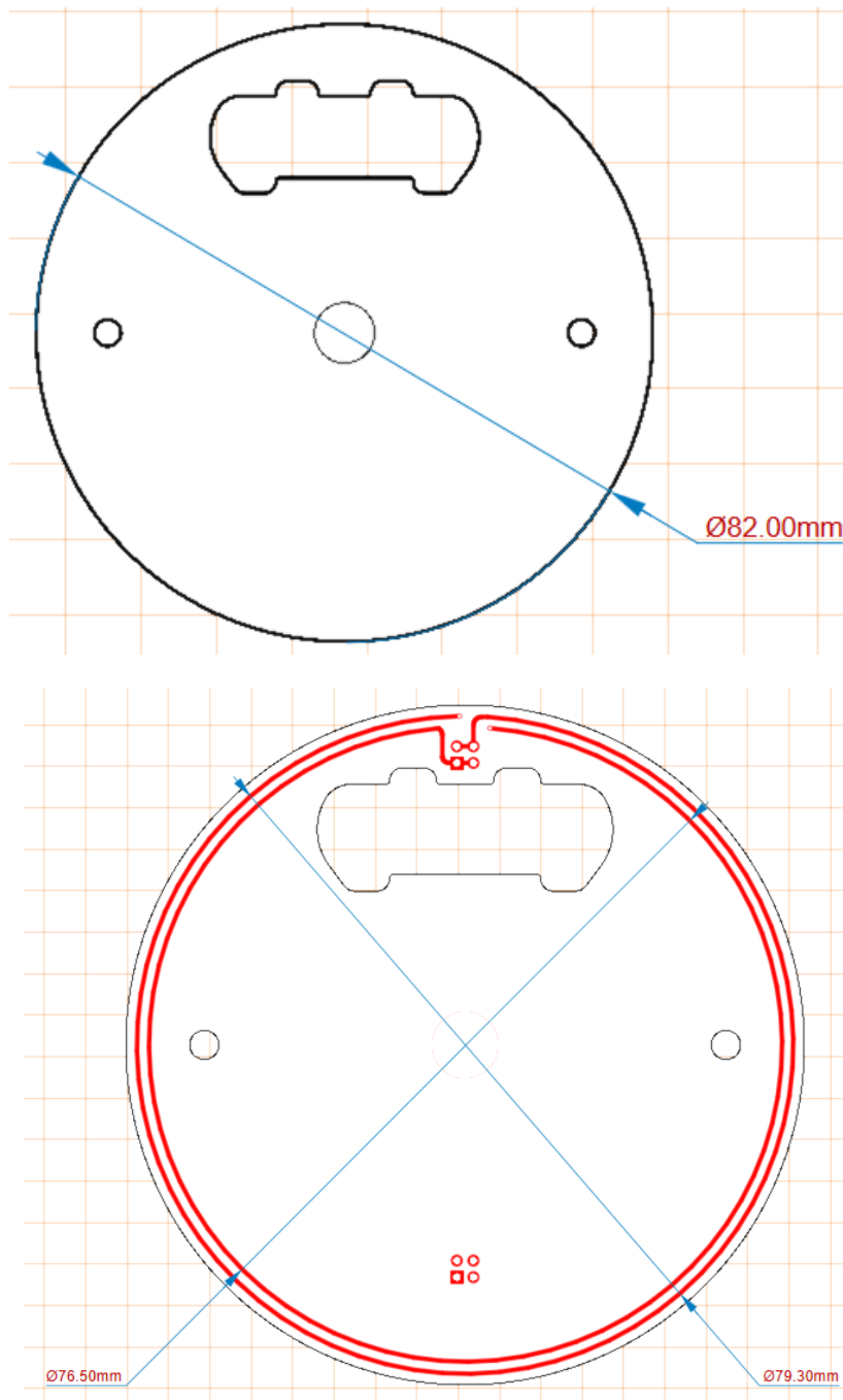
Figure 47: NFC Antenna Size
