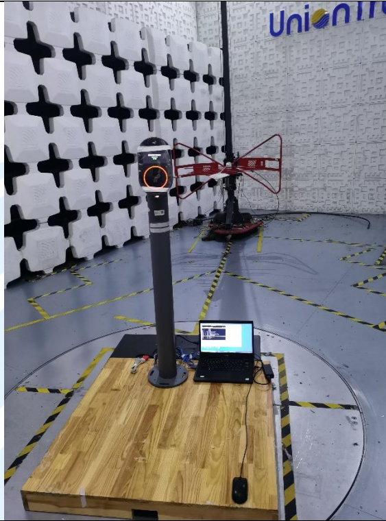
Radiated emission Test Setup-1 (30 MHz~1 GHz)
