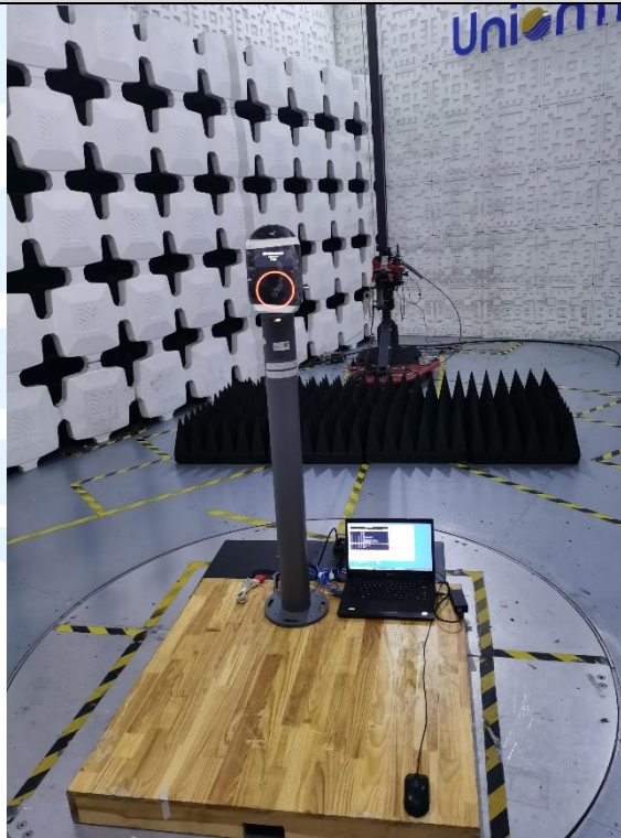
Radiated emission Test Setup-2 (Above 1 GHz)
