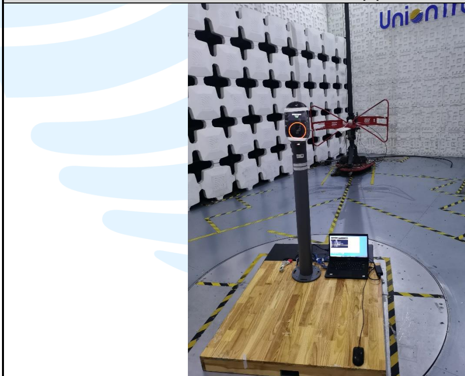
Radiated emission Test Setup (30 MHz~1 GHz)
