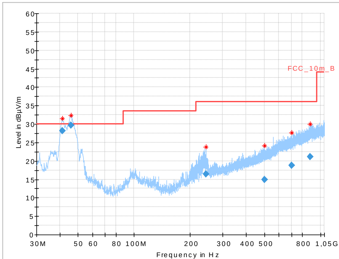
Plot 8: 30 MHz to 1 GHz, TX mode, middle channel, vertical & horizontal polarization, metal housing, adapter (non-Ex – version)
