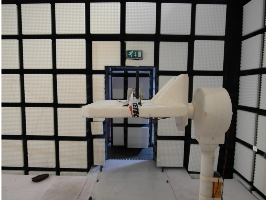
Photo 17: EUT at the anechoic chamber, metal housing (non-ex version)
