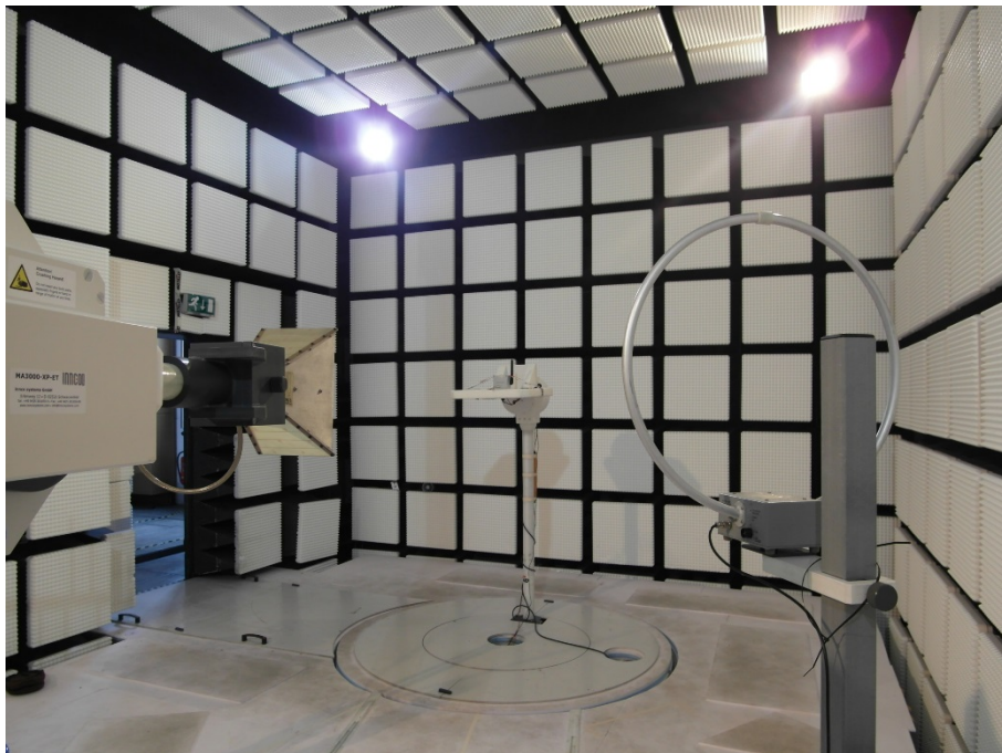
Photo 22: EUT at the anechoic chamber, metal housing (non-ex version)
