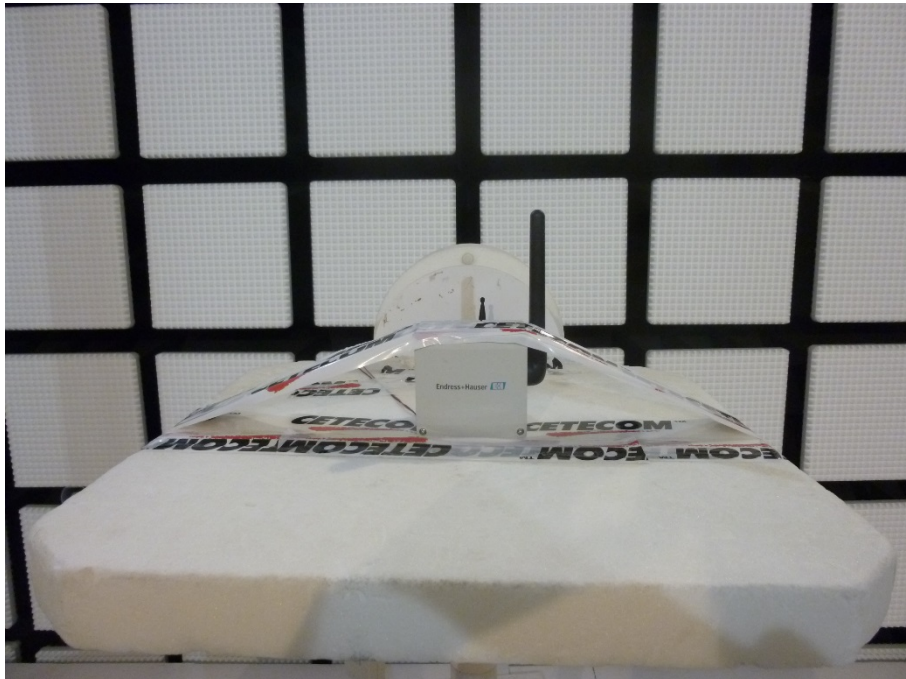
Photo 2: EUT at the anechoic chamber, plastic housing (ex version)
