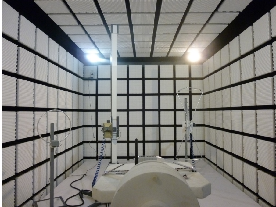
Photo 11: EUT at the anechoic chamber, metal housing (ex version)
