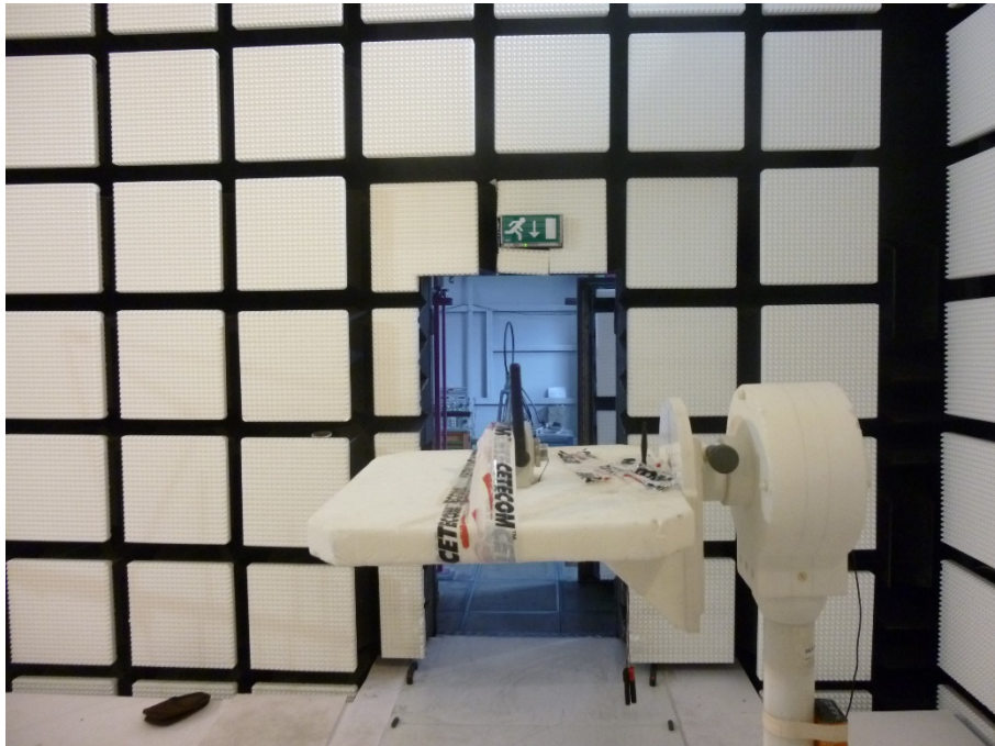
Photo 10: EUT at the anechoic chamber, metal housing (ex version)
