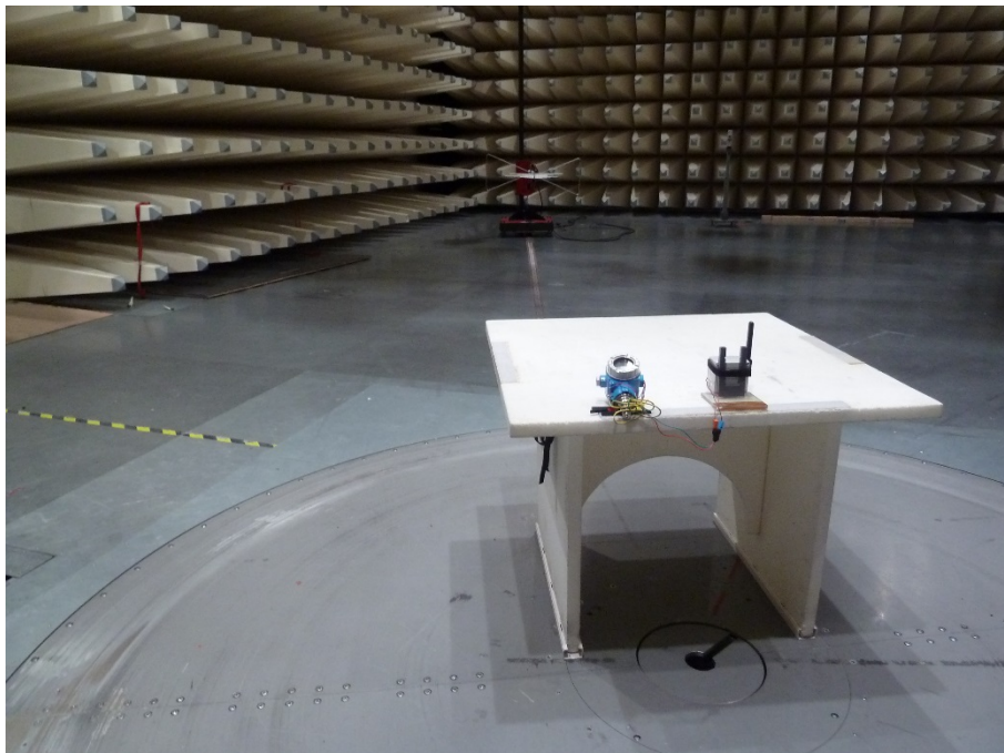
Photo 14: EUT at the semi-anechoic chamber, metal housing (ex version)
