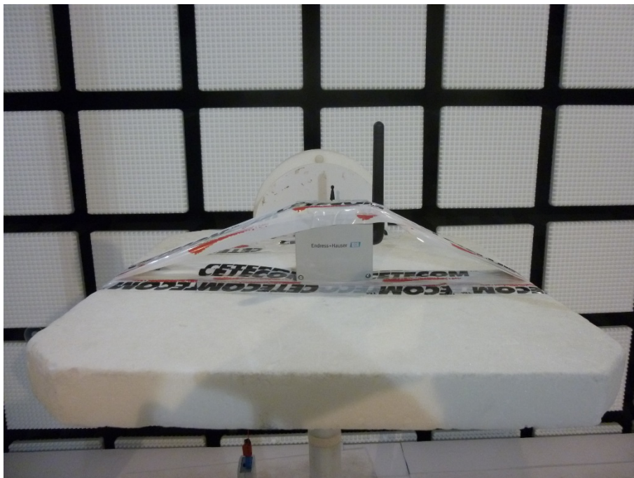
Photo 8: EUT at the anechoic chamber, metal housing (ex version)
