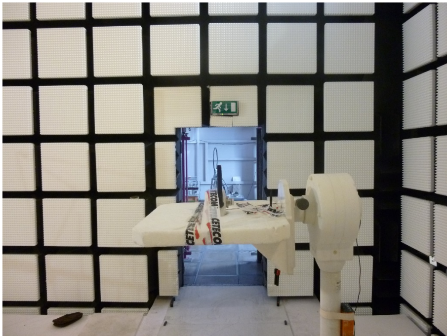
Photo 4: EUT at the anechoic chamber, plastic housing (ex version)
