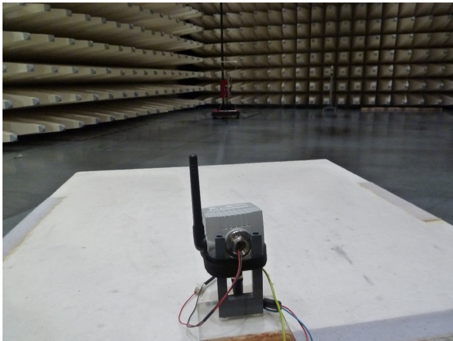
Photo 24: EUT at the semi-anechoic chamber, metal housing (non-ex version)
