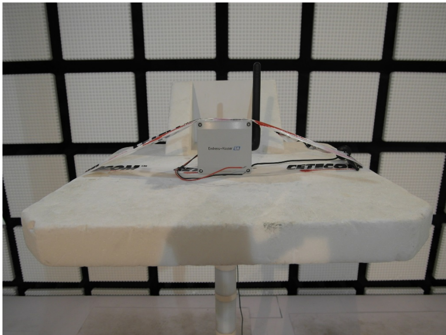
Photo 18: EUT at the anechoic chamber, metal housing (non-ex version)
