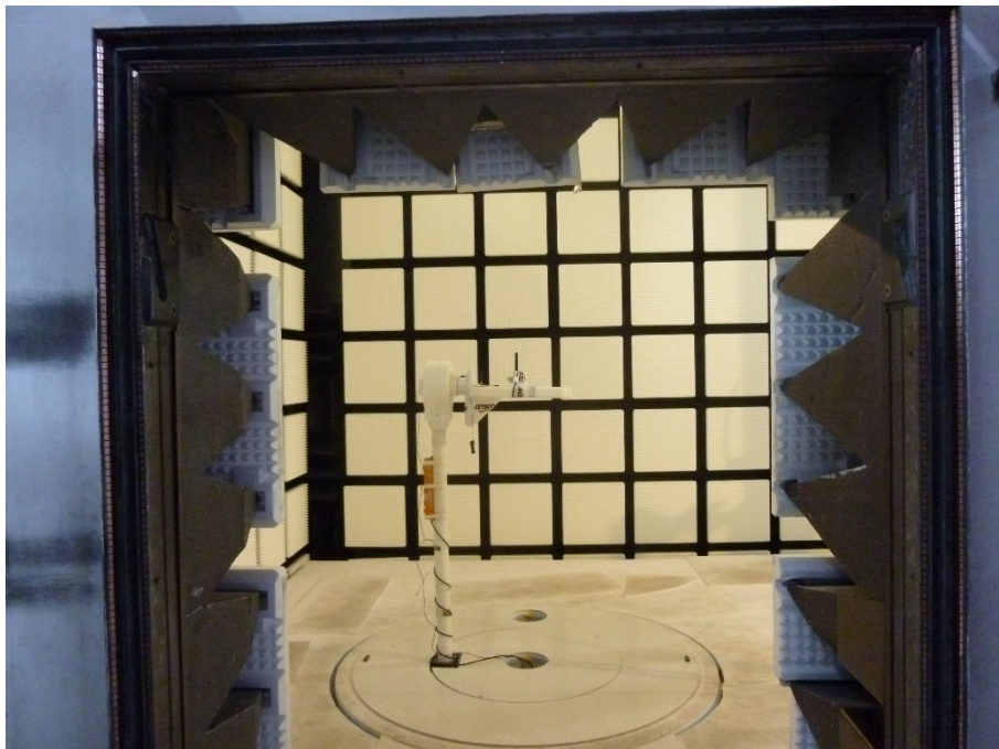
Photo 6: EUT at the anechoic chamber, plastic housing (ex version)
