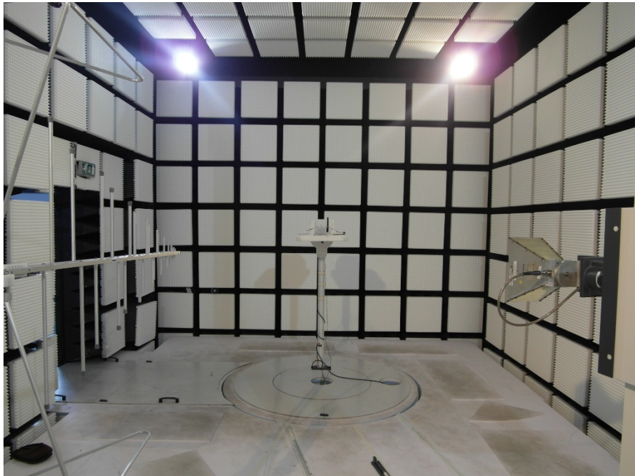
Photo 20: EUT at the anechoic chamber, metal housing (non-ex version)
