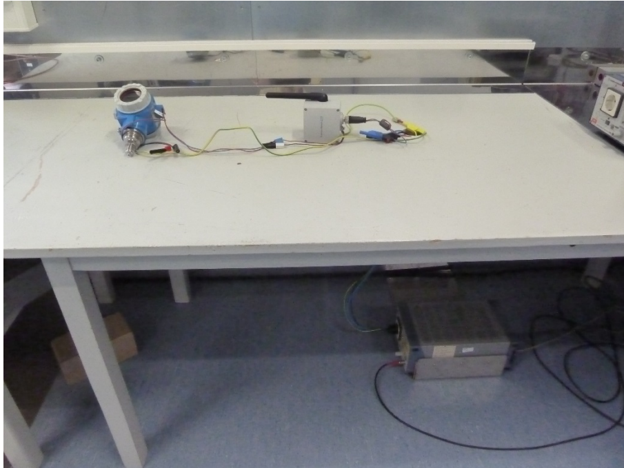
Photo 25: AC conducted, metal housing (non-ex version)
