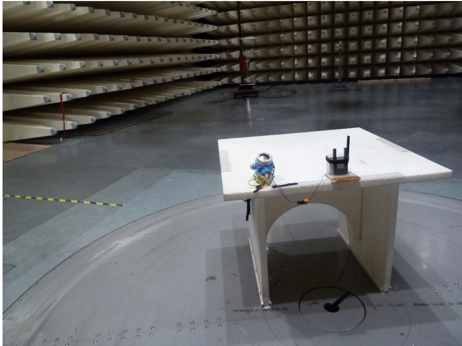
Photo 7: EUT at the semi-anechoic chamber, plastic housing (ex version)
