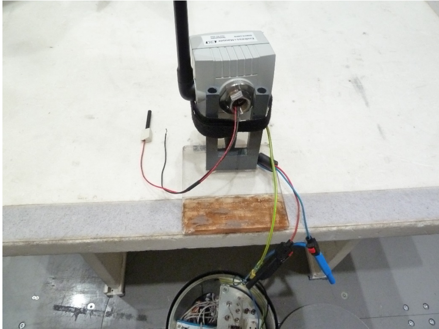
Photo 23: EUT at the semi-anechoic chamber, metal housing (non-ex version)
