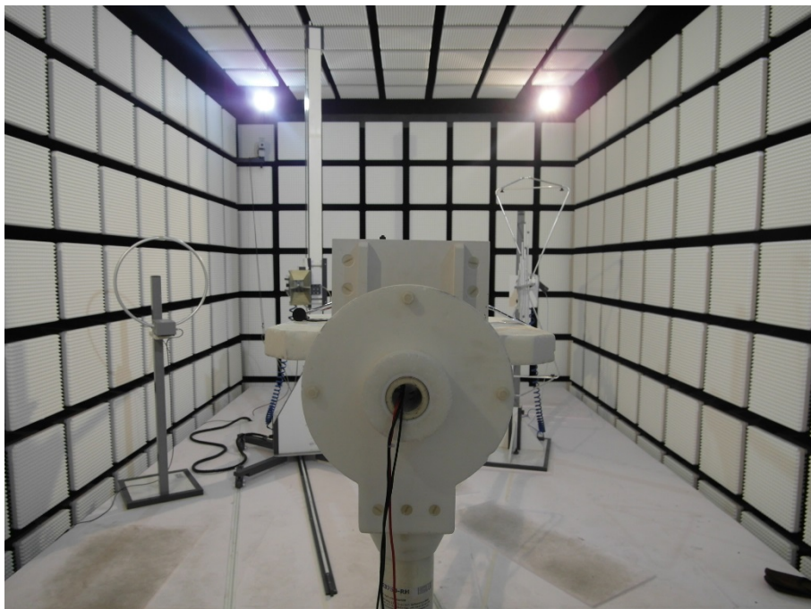
Photo 16: EUT at the anechoic chamber, metal housing (non-ex version)
