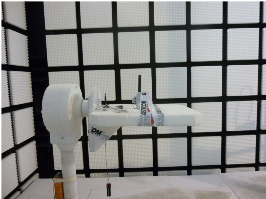
Photo 12: EUT at the anechoic chamber, metal housing (ex version)
