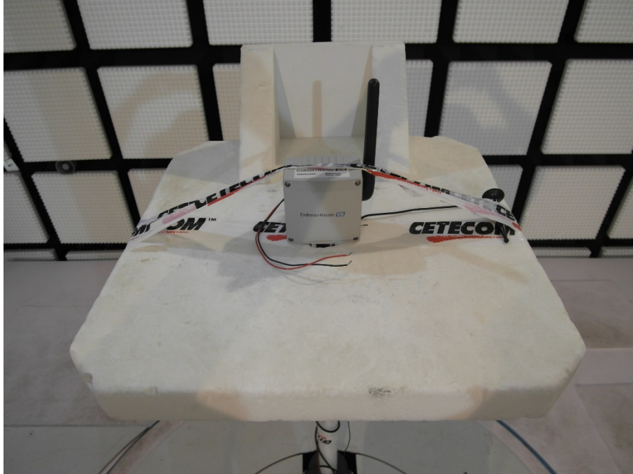
Photo 19: EUT at the anechoic chamber, metal housing (non-ex version)
