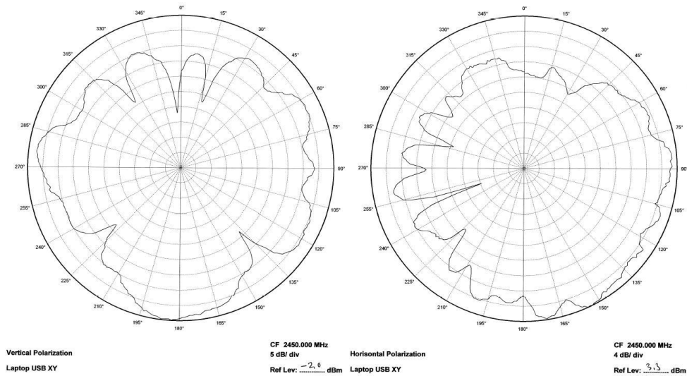
EFFICIENCY/GAIN TEST
