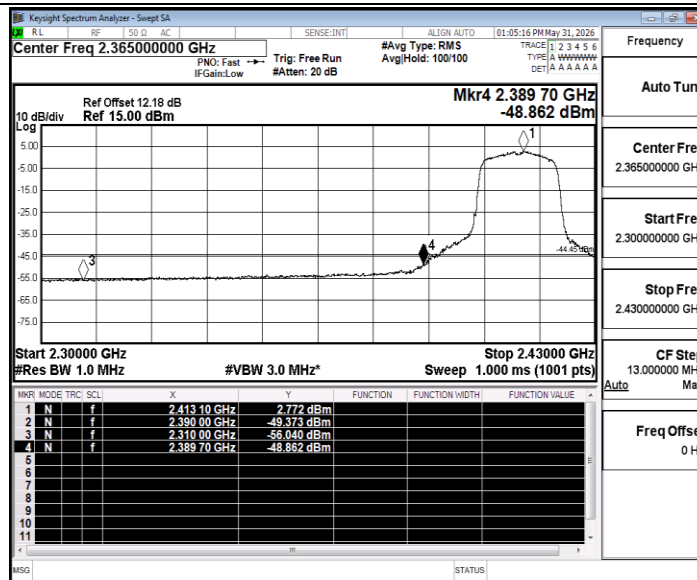
11N20SISO_Ant2_Low_2412_Peak
