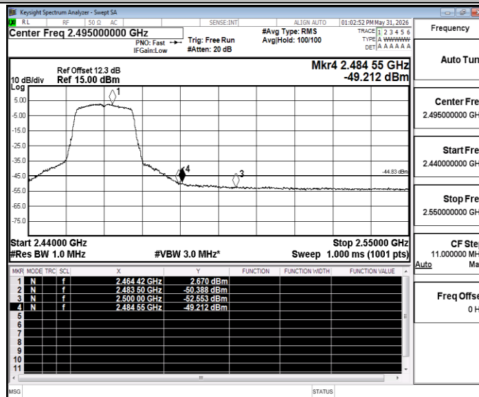
11G_Ant2_High_2462_Peak
