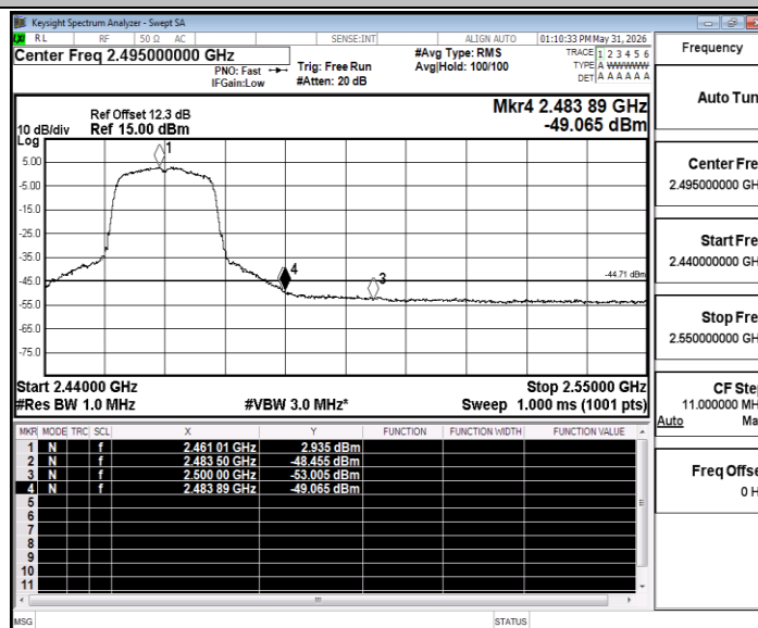
11N20SISO_Ant2_High_2462_Peak
