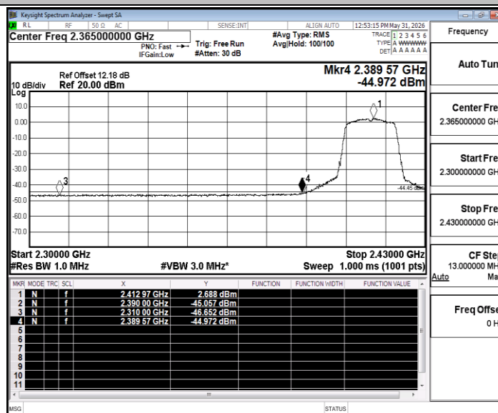
11G_Ant2_Low_2412_Peak
