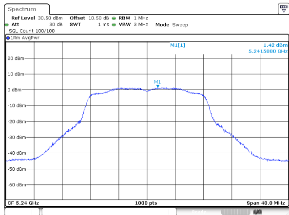
802.11a_5240MHz_ANT 1
