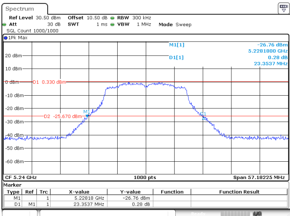
802.11a_5240MHz_ANT 2
