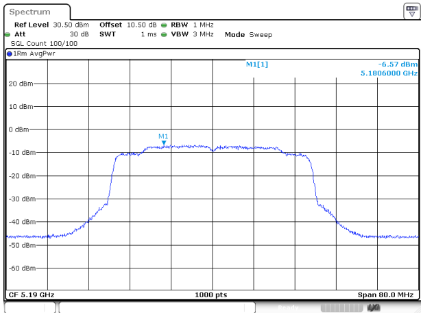
802.11ac40_5190MHz_ANT 2
