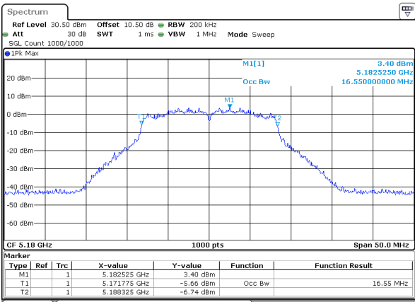
802.11a_5180MHz_ANT 1
