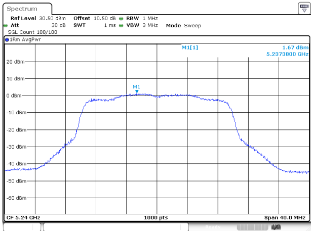
802.11ac20_5240MHz_ANT 1
