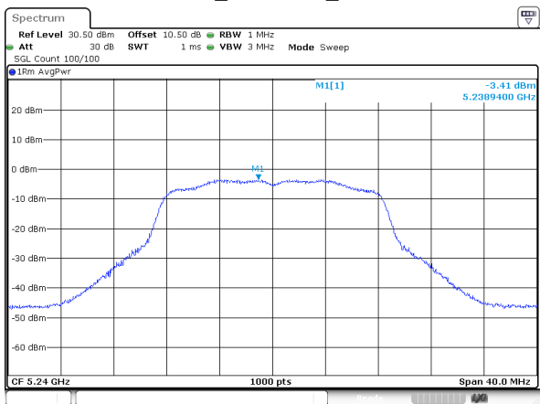
802.11a_5240MHz_ANT 2
