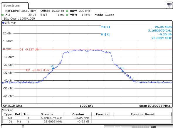
802.11a_5180MHz_ANT 2
