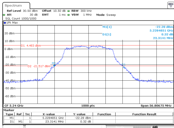
802.11a_5240MHz_ANT 1
