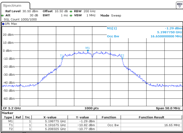
802.11a_5200MHz_ANT 2
