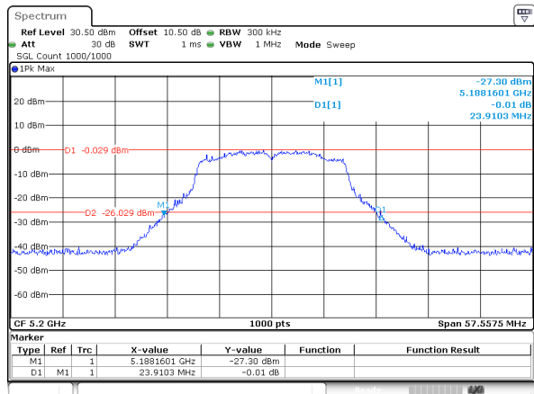
802.11a_5200MHz_ANT 2
