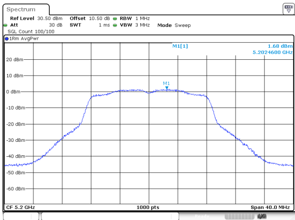
802.11a_5200MHz_ANT 1
