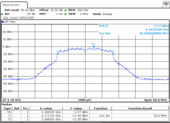
802.11a_5180MHz_ANT 2
