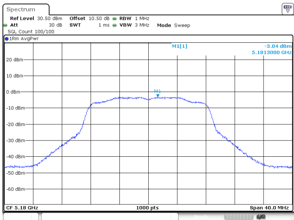
802.11a_5180MHz_ANT 2
