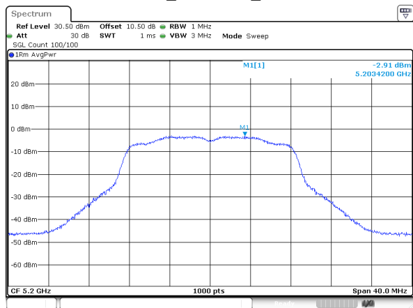
802.11a_5200MHz_ANT 2
