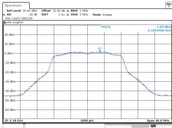
802.11a_5180MHz_ANT 1
