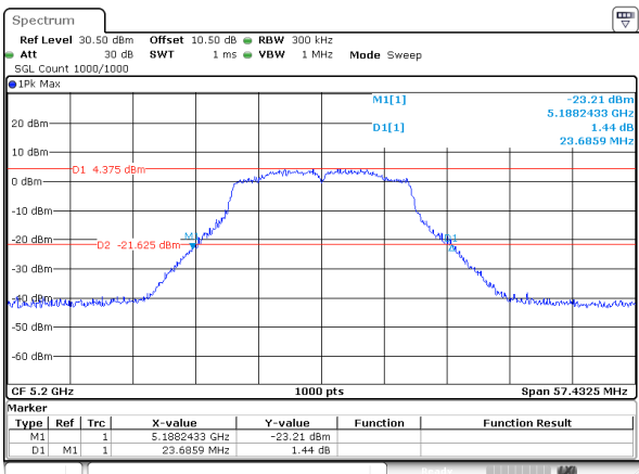
802.11a_5200MHz_ANT 1
