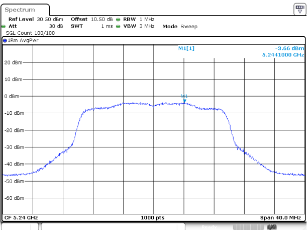
802.11ac20_5240MHz_ANT 2
