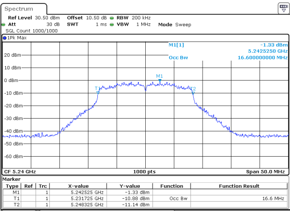
802.11a_5240MHz_ANT 2
