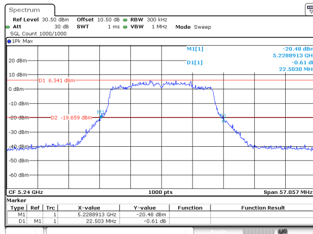
802.11ac20_5240MHz_ANT 1
