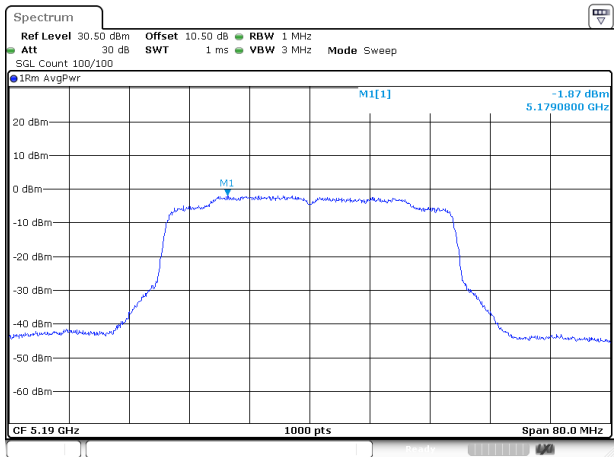
802.11ac40_5190MHz_ANT 1
