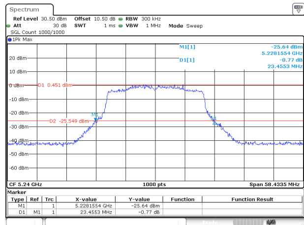
802.11ac20_5240MHz_ANT 2
