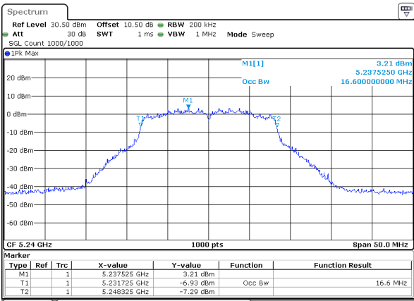
802.11a_5240MHz_ANT 1
