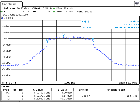
802.11a_5200MHz_ANT 1
