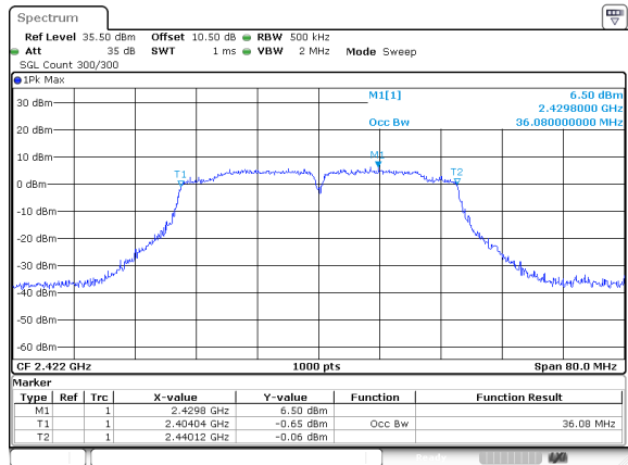
802.11n40_2422MHz_ANT 2
