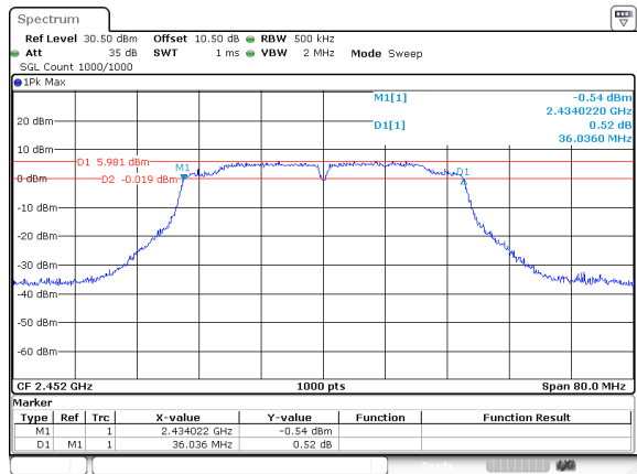
802.11n40_2452MHz_ANT 2
