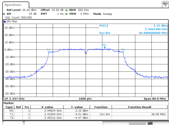
802.11n40_2437MHz_ANT 1
