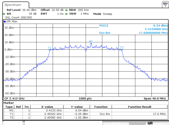
802.11n20_2412MHz_ANT 2
