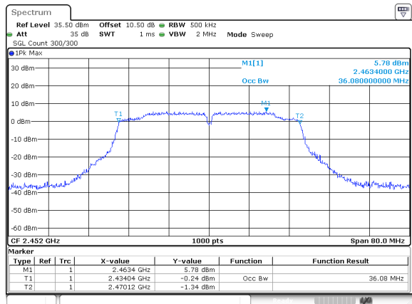
802.11n40_2452MHz_ANT 2
