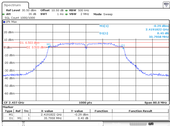
802.11n40_2437MHz_ANT 2
