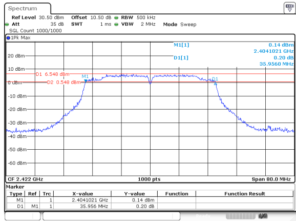
802.11n40_2422MHz_ANT 2
