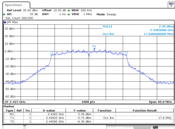
802.11n20_2437MHz_ANT 1
