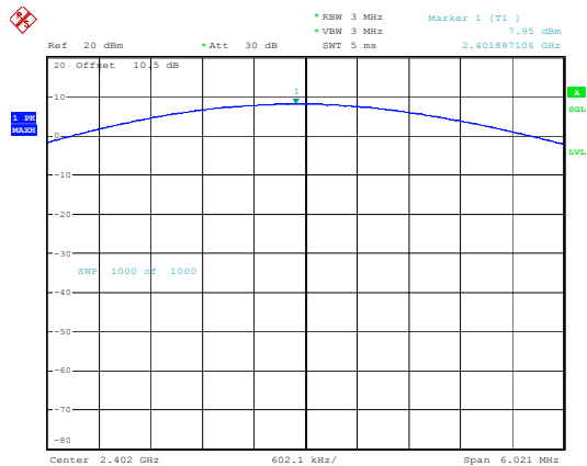
EDR(8DPSK)_3DH1_Low
