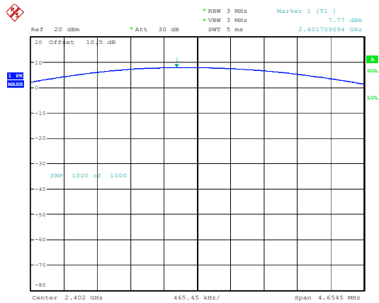
BDR(GFSK)_DH1_Low
