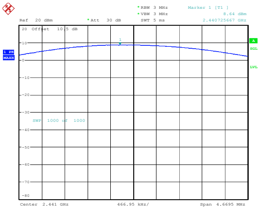
BDR(GFSK)_DH1_Middle
