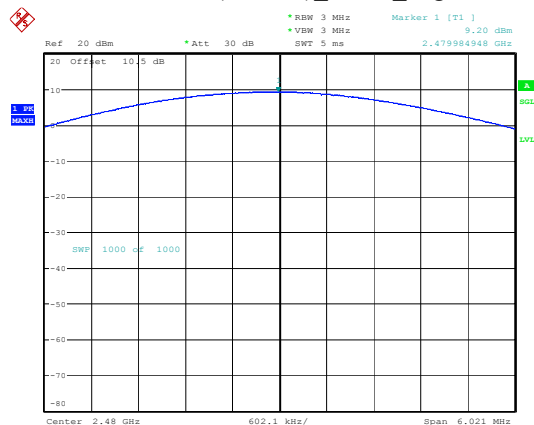
EDR(8DPSK)_3DH1_High
