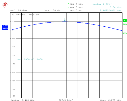
EDR(8DPSK)_3DH1_Additional
