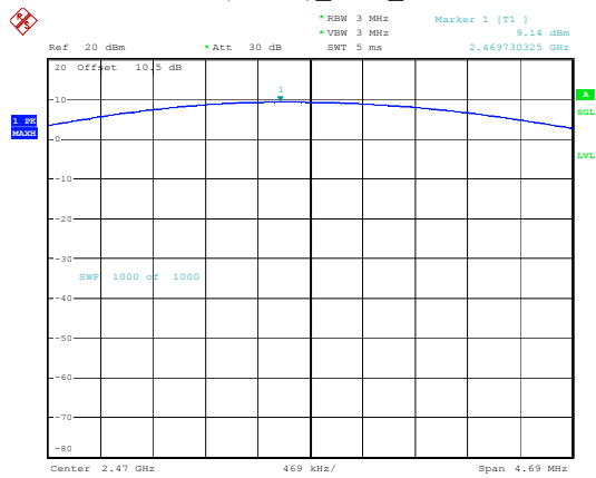
BDR(GFSK)_DH1_Additional
