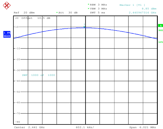
EDR(8DPSK)_3DH1_Middle
