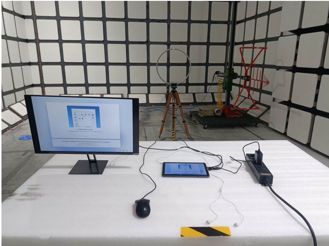
Radiated Emissions View (Below 1 GHz)_fast charge
