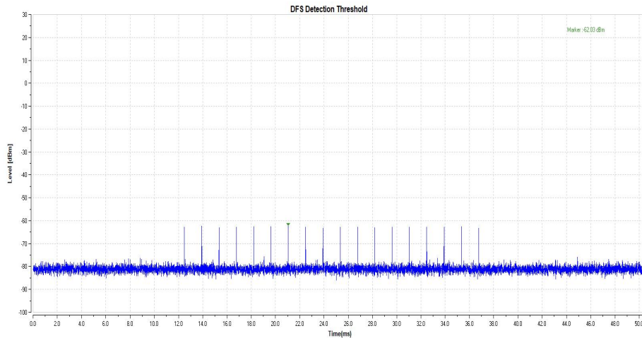
Radar Singal 0
