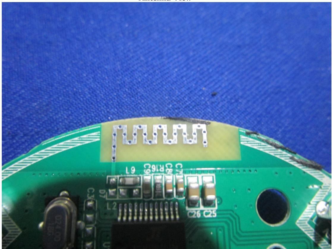
Antenna View
