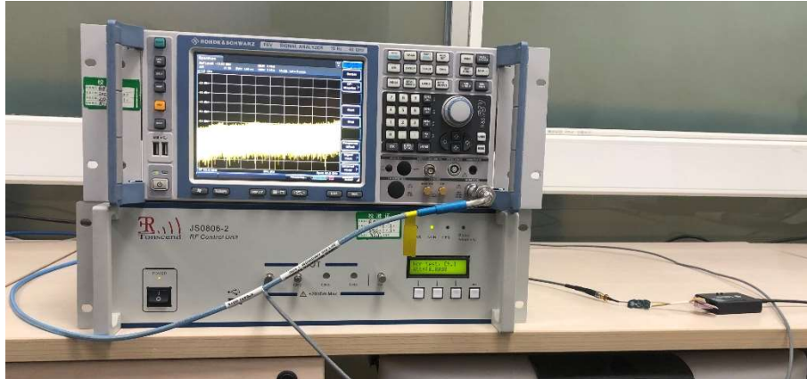
RF Conducted Test Setup
