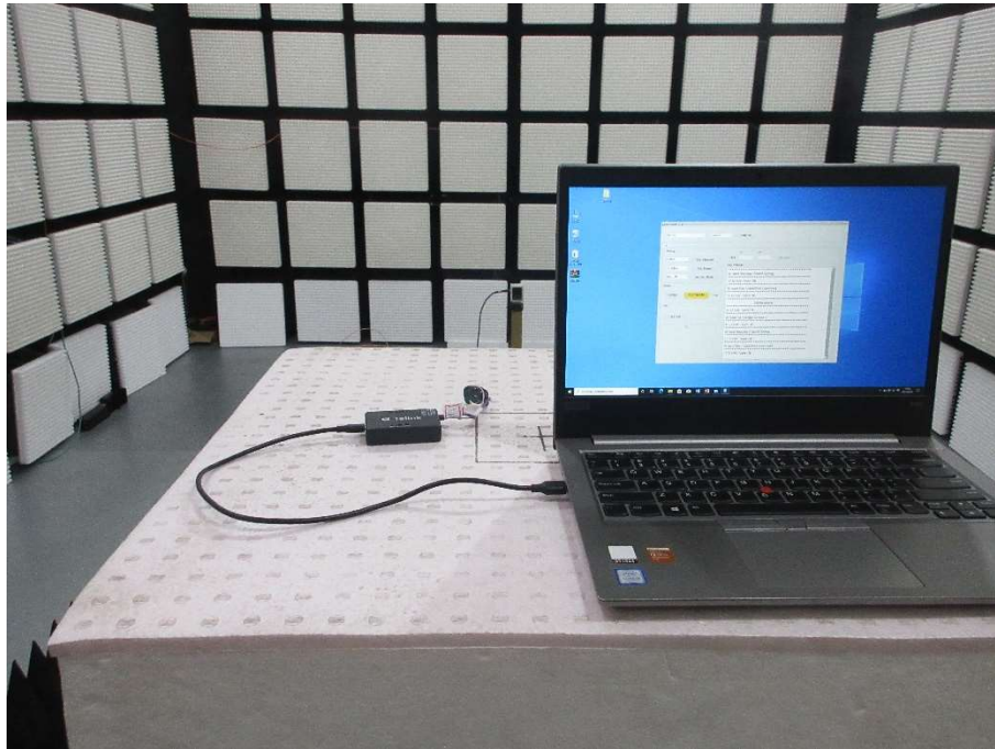
Spurious Radiated Emissions Test Setup (Above 18GHz)
