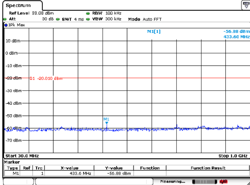
(Plot 4.9.1 A1: Channel 00: 2402MHz @ GFSK)
