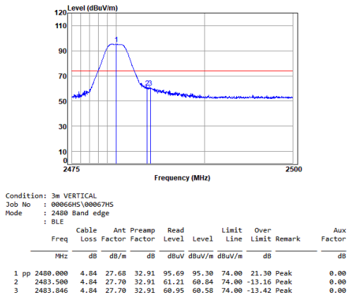
BLE_2M_TX_CH_39_Vertical-Peak
