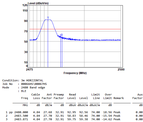
BLE_2M_TX_CH_39_Horizontal-Peak
