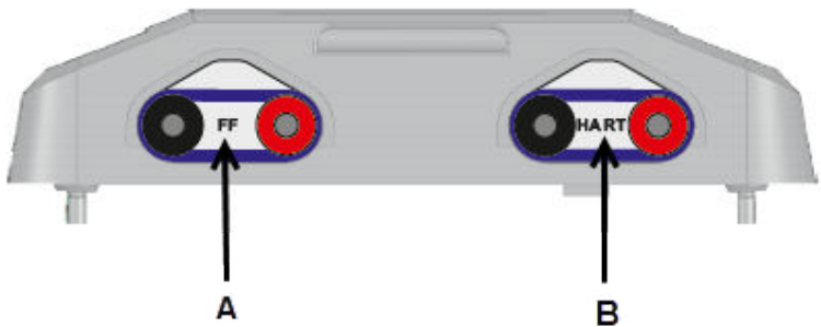
Figure 1-2: Device Communicator communication module
