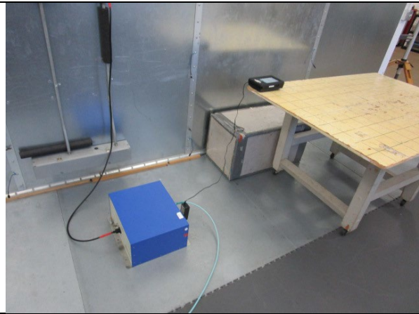
AC Mains Conducted Emissions setup
