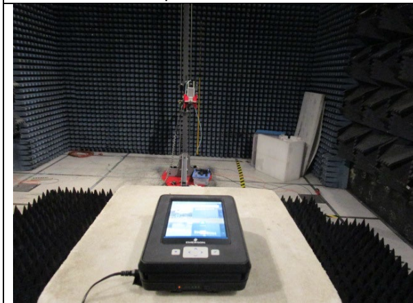
1-4GHz setup
