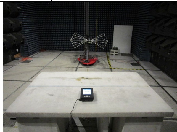
30-200MHz setup
