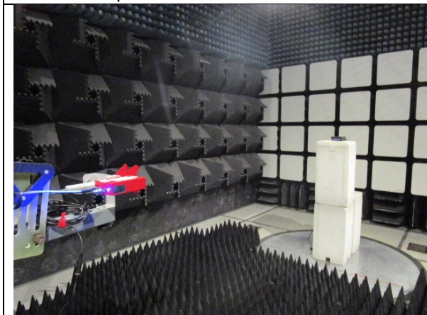
18-25GHz setup
