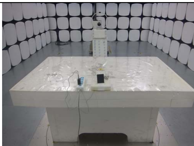
Radiated Spurious Emissions Test Setup 0.1MHz-30MHz
