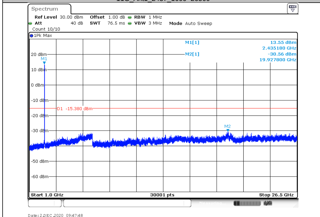
11G_Ant1_2437_1000~26500
