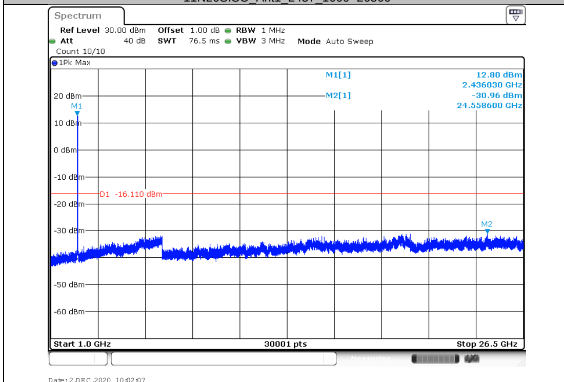
11N20SISO_Ant1_2437_1000~26500
