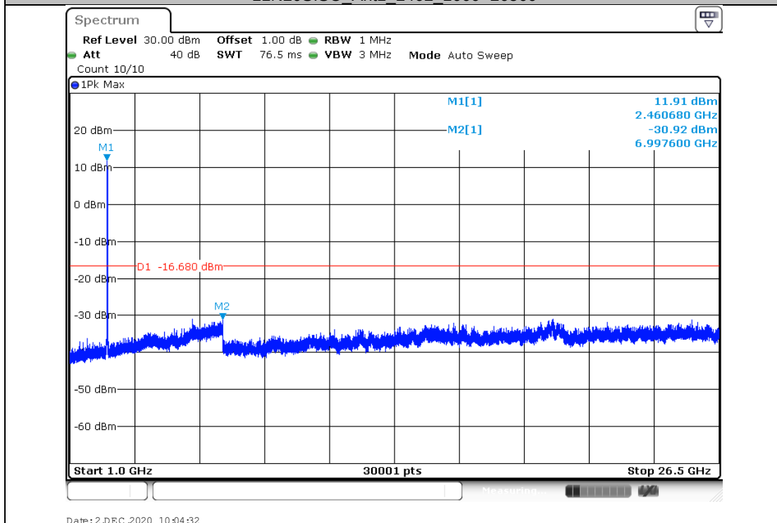
11N20SISO_Ant1_2462_1000~26500
