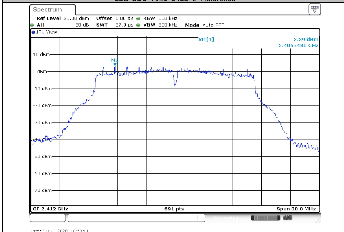
11G-CDD_Ant1_2412_0~Reference
