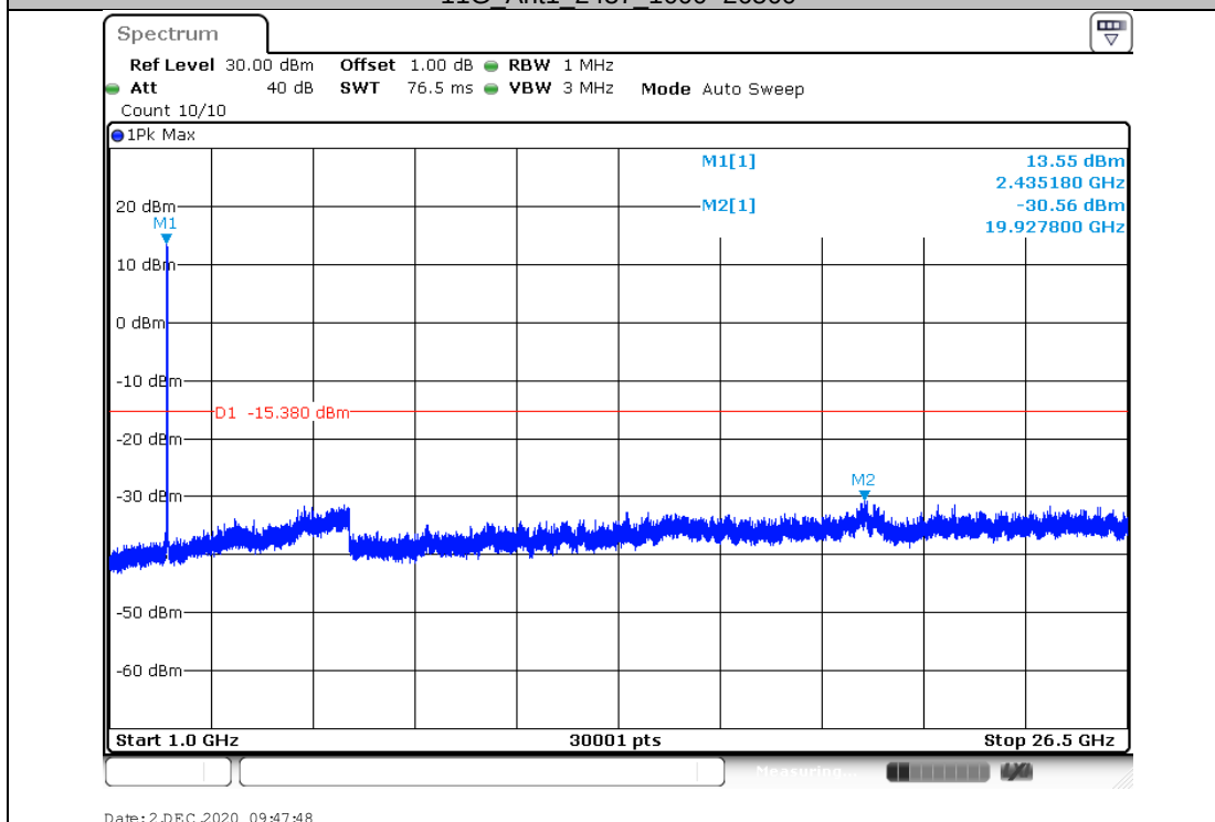
11G_Ant1_2437_1000~26500
