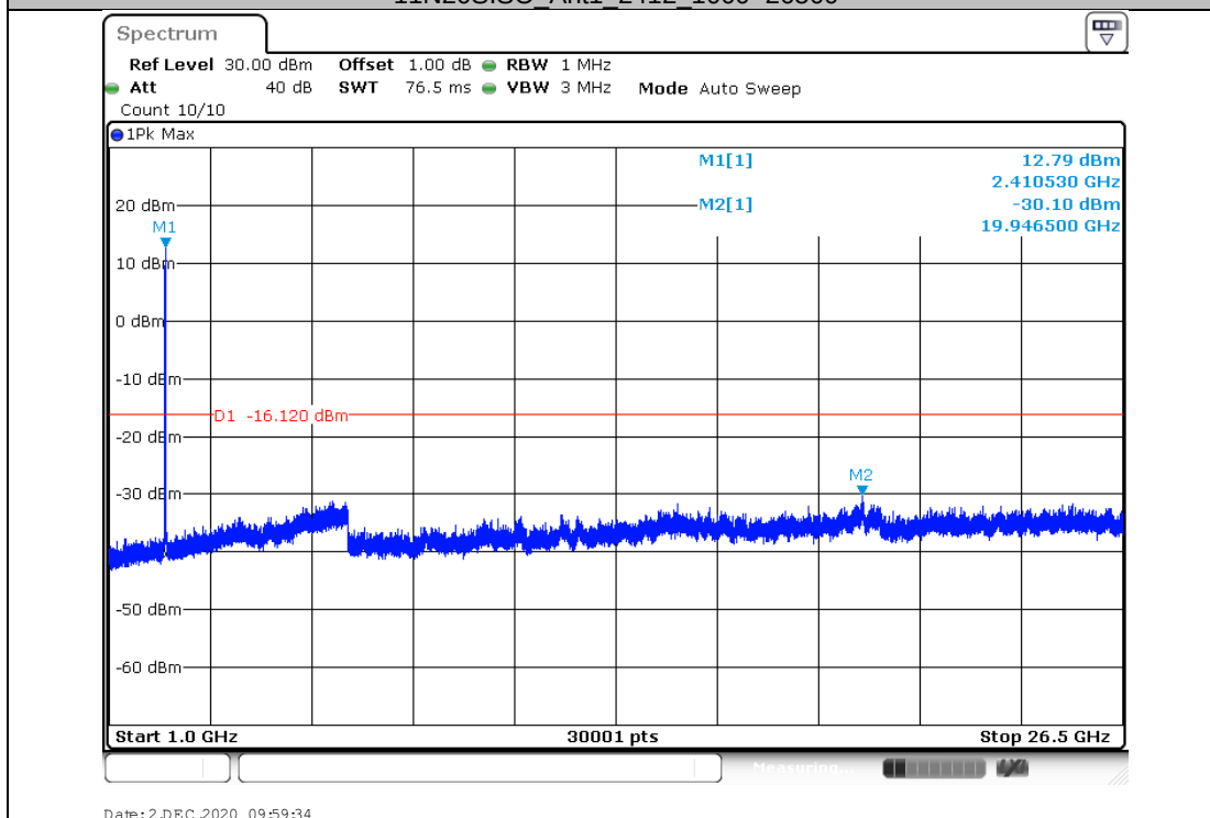
11N20SISO_Ant1_2412_1000~26500
