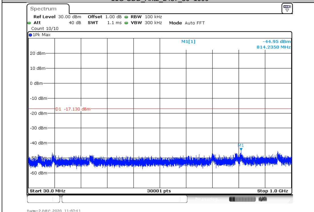
11G-CDD_Ant2_2437_30~1000
