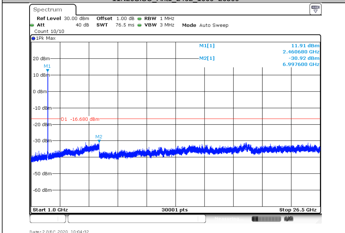
11N20SISO_Ant1_2462_1000~26500
