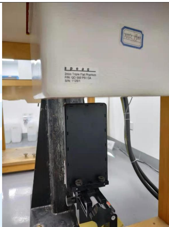
Bottom Side of EUT with 1.0 cm Gap
