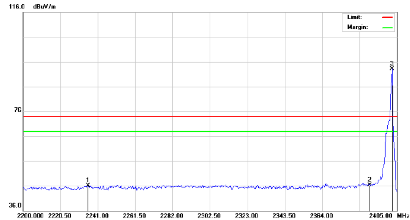
TEST PLOT OF BAND EDGE FOR LOW CHANNEL (2Mbps)-Horizontal
