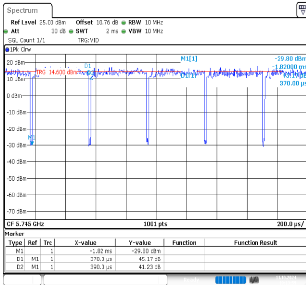
NTNV-11AC20MIMO-Ant1-5745
