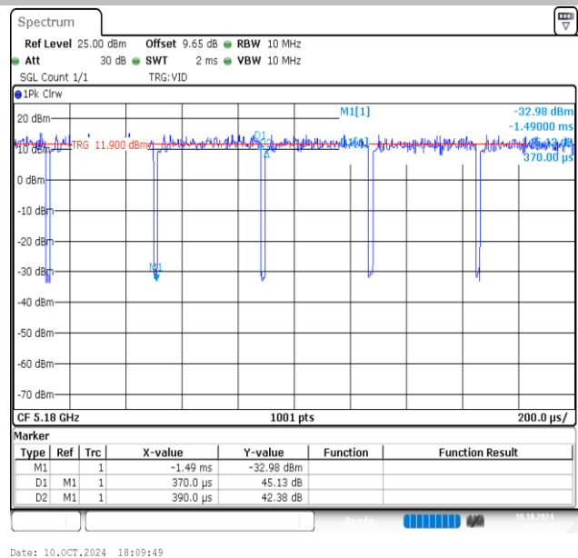
NTNV-11AC20MIMO-Ant2-5180
