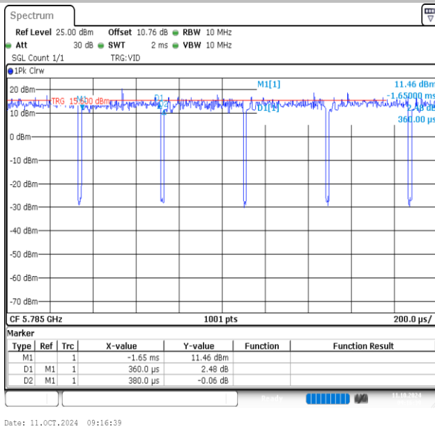
NTNV-11AC20MIMO-Ant1-5785
