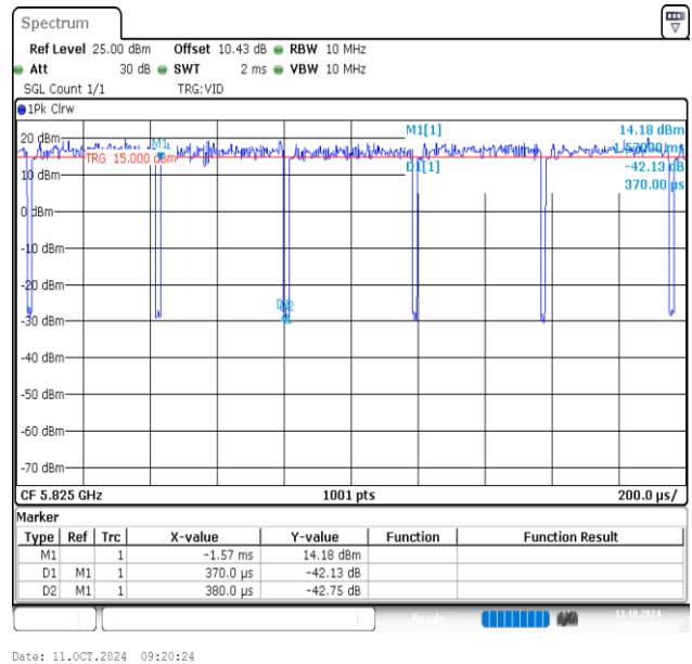
NTVN-11AC20MIMO-Ant2-5825
