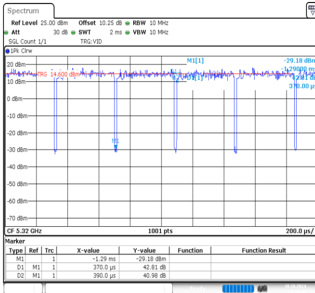
NTNV-11AC20MIMO-Ant1-5320
