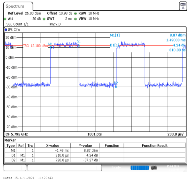
NTNV-11N40MIMO-Ant2-5795
