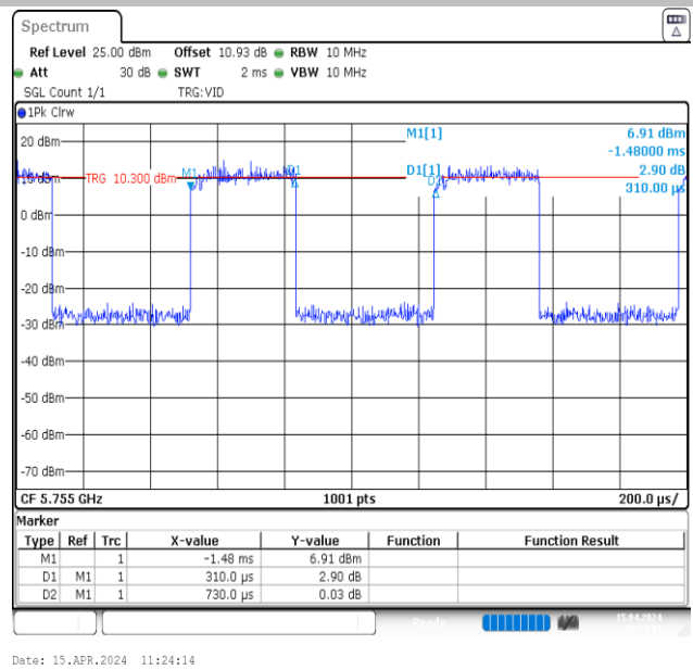
NTNV-11N40MIMO-Ant2-5755
