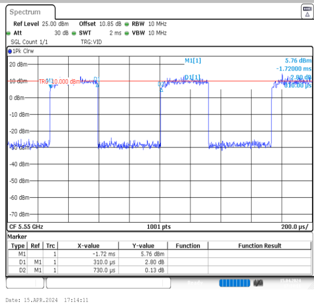
NTNV-11N40MIMO-Ant2-5550
