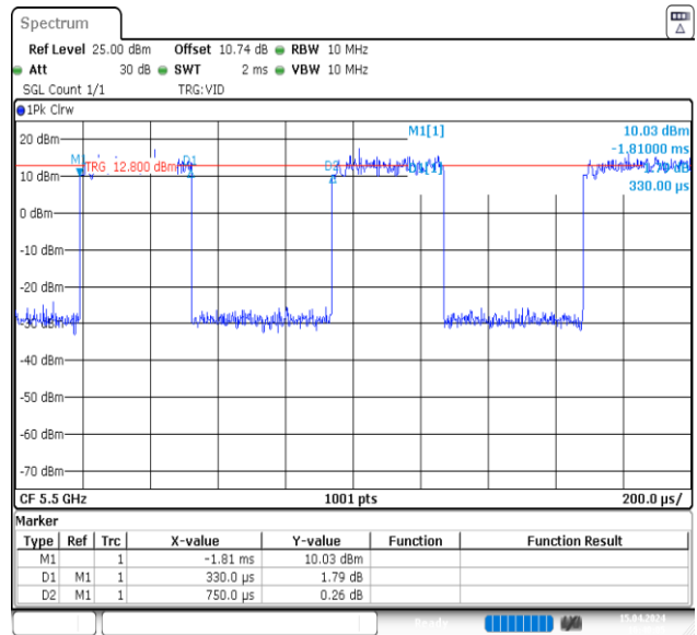
NTNV-11N20MIMO-Ant2-5500
