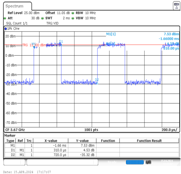
NTNV-11N40MIMO-Ant2-5670
