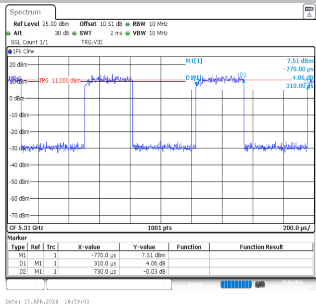
NTNV-11N40MIMO-Ant2-5310
