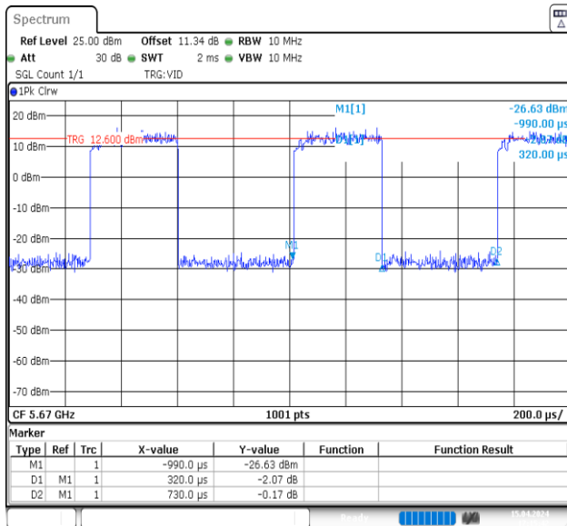
NTNV-11N40MIMO-Ant1-5670
