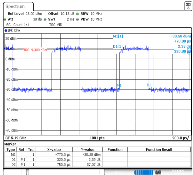
NTNV-11N40MIMO-Ant2-5190
