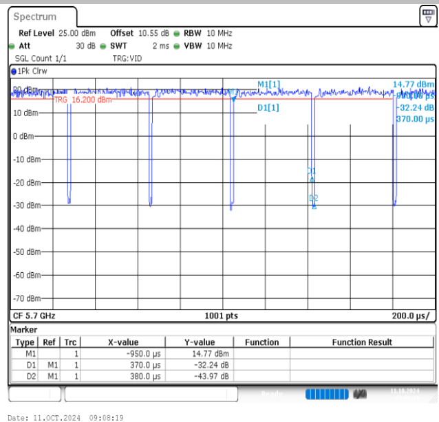
NTNV-11AC20MIMO-Ant2-5700
