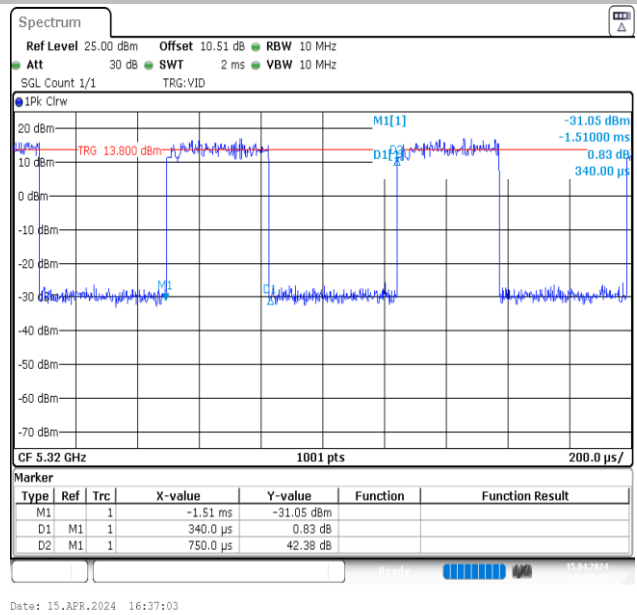
NTNV-11N20MIMO-Ant2-5320
