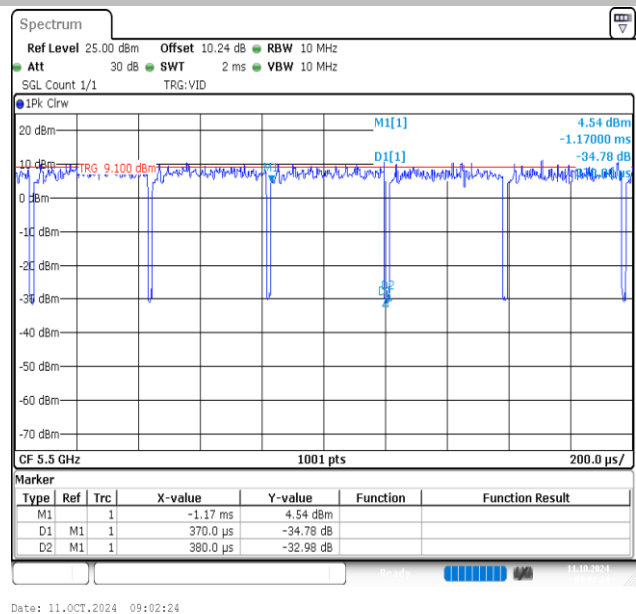
NTNV-11AC20MIMO-Ant2-5500
