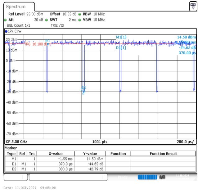
NTNV-11AC20MIMO-Ant2-5580
