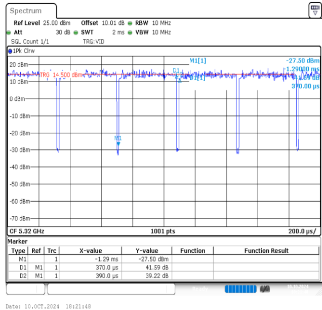
NTNV-11AC20MIMO-Ant2-5320
