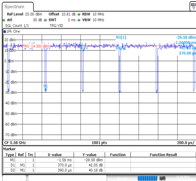
NTNV-11AC20MIMO-Ant1-5580
