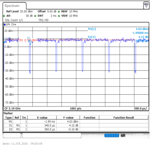
NTVN-11AC40MIMO-Ant2-5190
