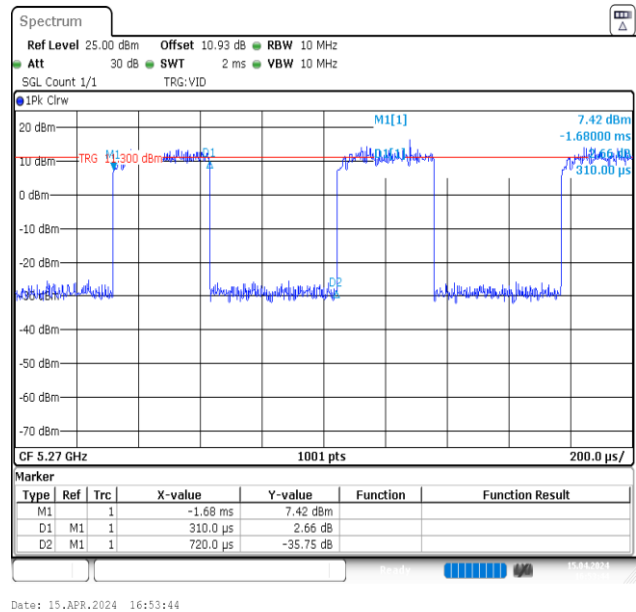
NTNV-11N40MIMO-Ant2-5270
