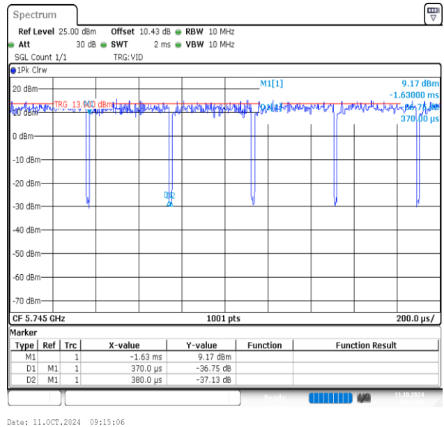
NTNV-11AC20MIMO-Ant2-5745
