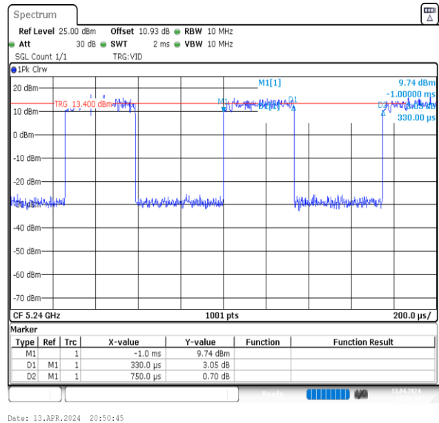
NTNV-11N20MIMO-Ant2-5240
