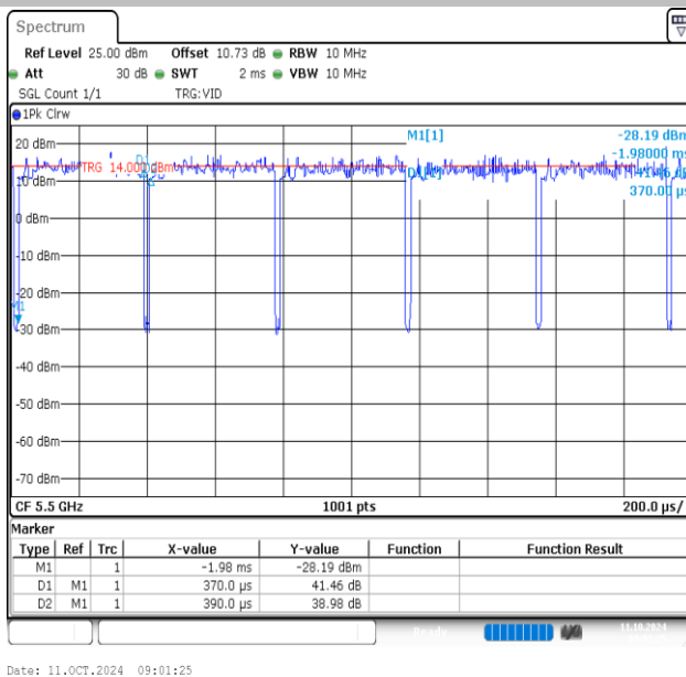
NTNV-11AC20MIMO-Ant1-5500
