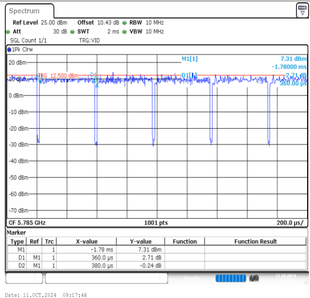
NTNV-11AC20MIMO-Ant2-5785
