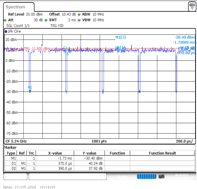
NTNV-11AC20MIMO-Ant2-5240
