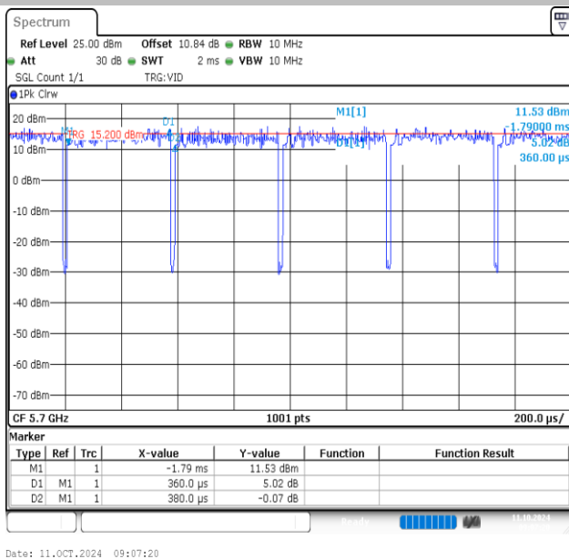
NTNV-11AC20MIMO-Ant1-5700
