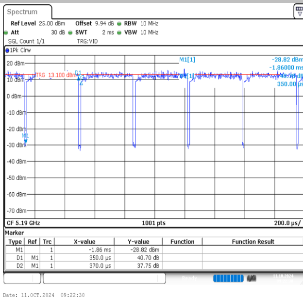
NTVN-11AC40MIMO-Ant1-5190
