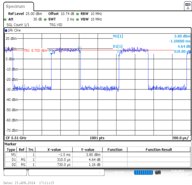
NTNV-11N40MIMO-Ant2-5510
