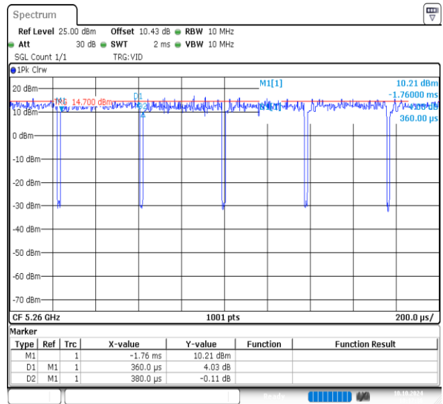
NTVN-11AC20MIMO-Ant2-5260
