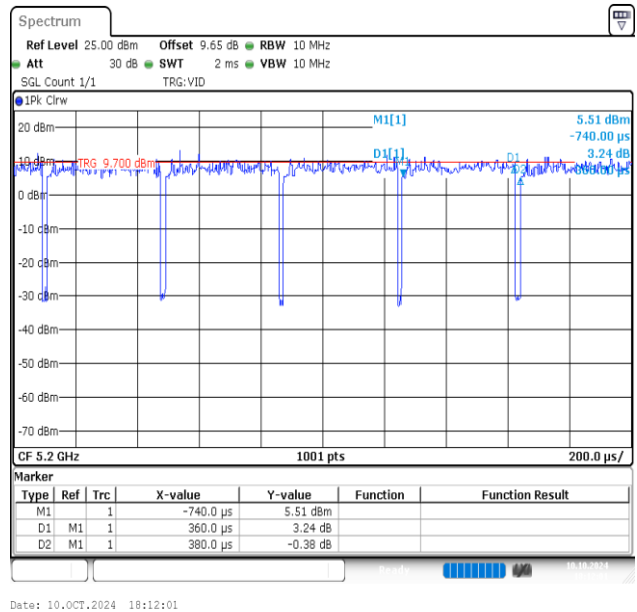
NTNV-11AC20MIMO-Ant2-5200
