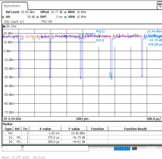
NTNV-11AC20MIMO-Ant1-5240
