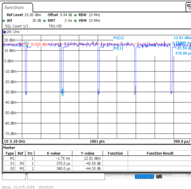
NTNV-11AC20MIMO-Ant1-5180
