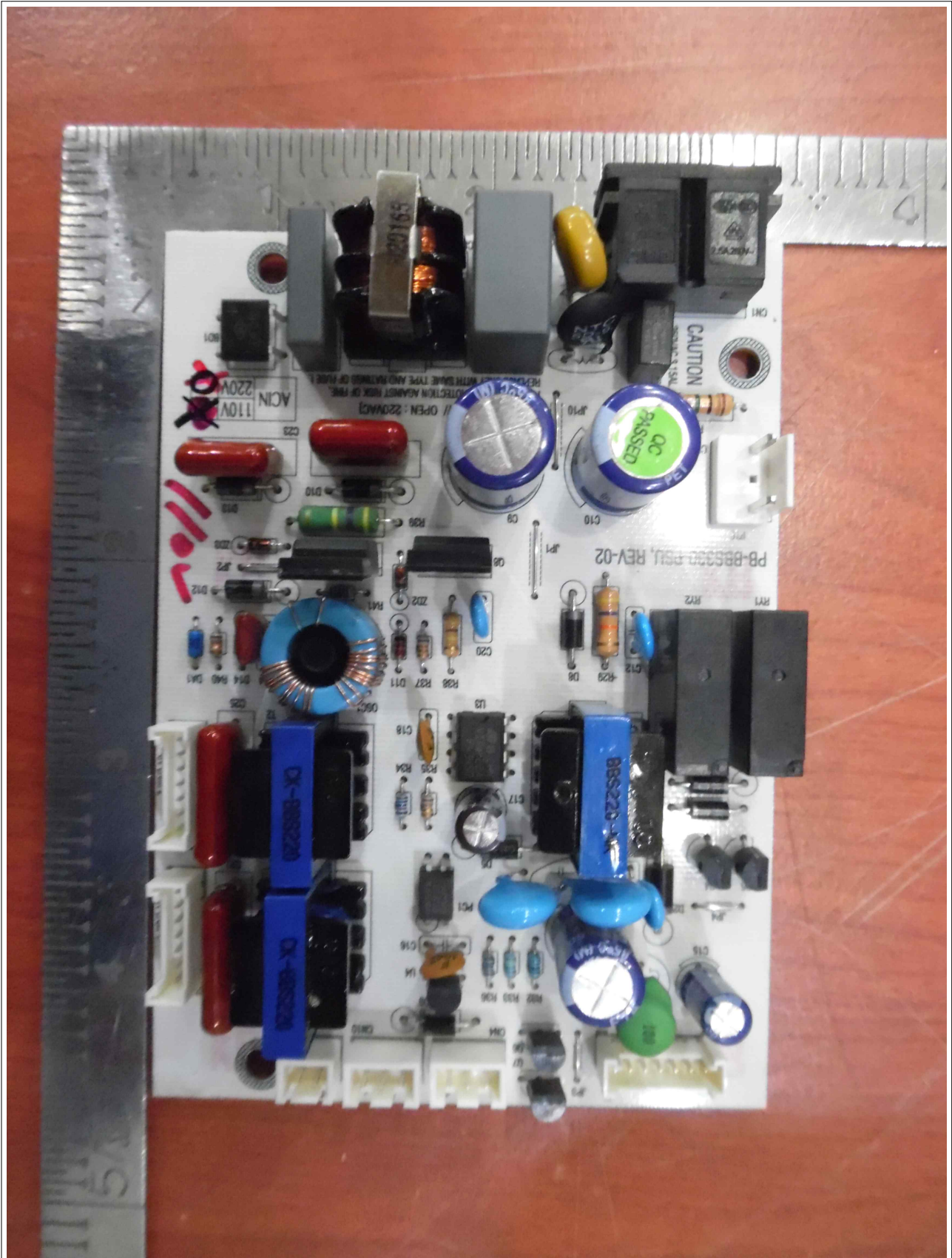
View of PCB(Top)
