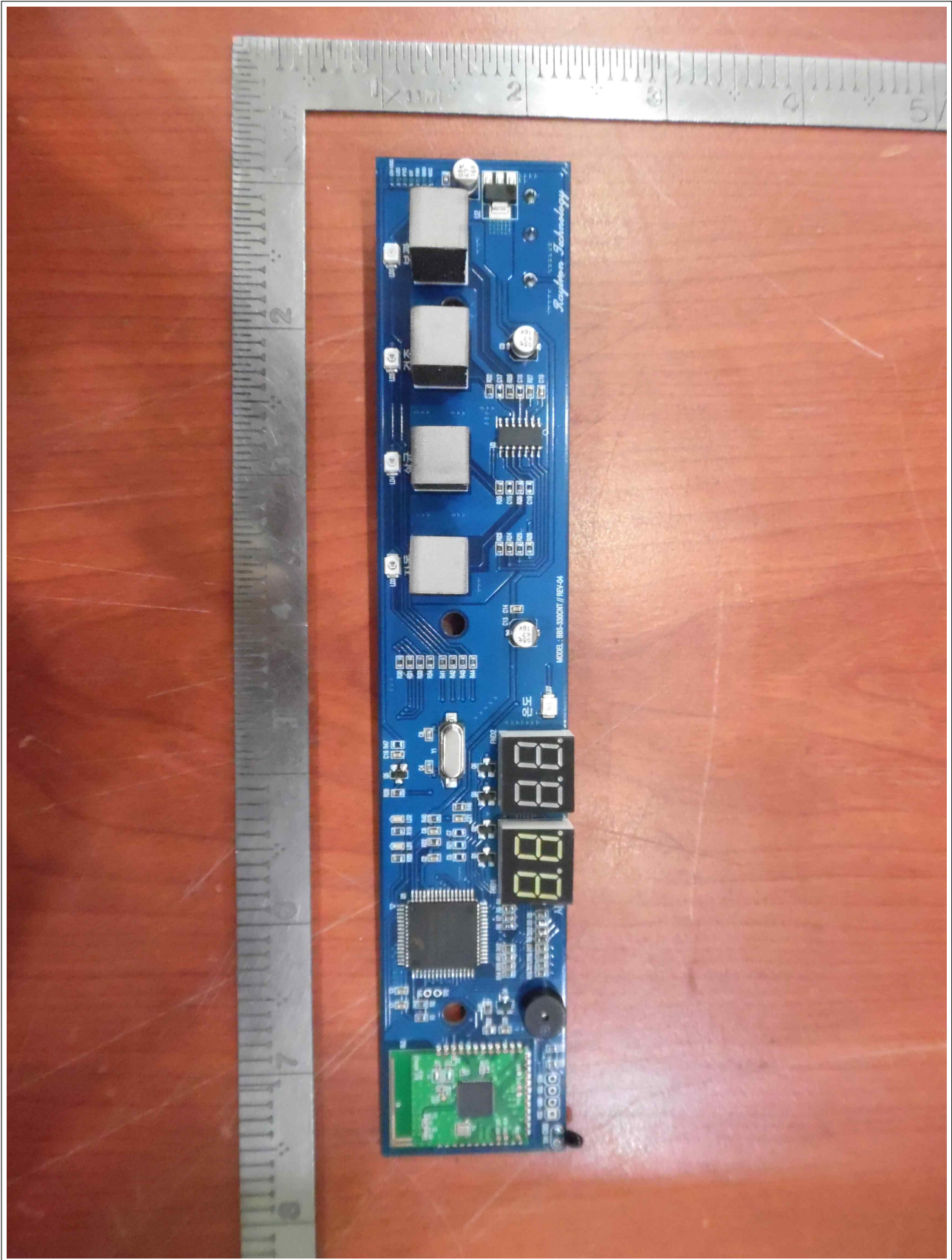
View of PCB2(Top)
