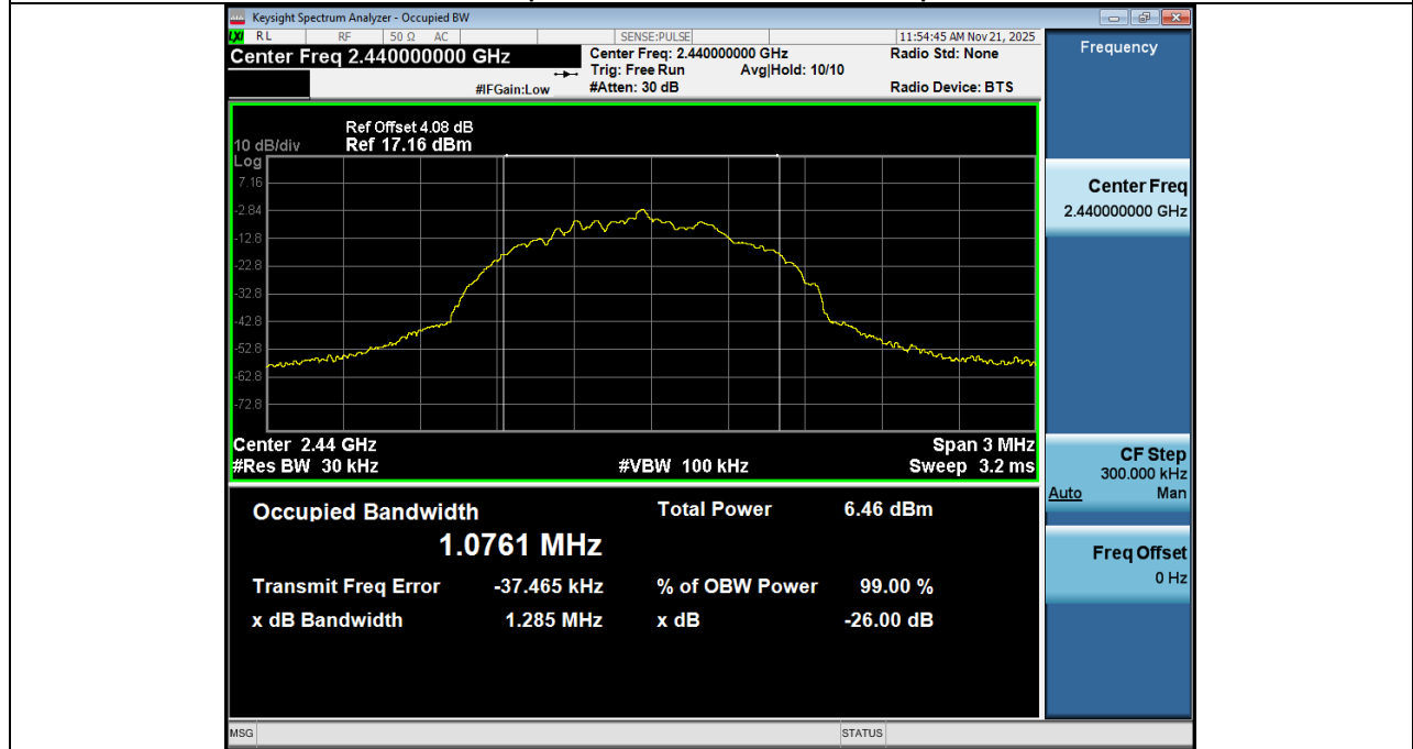
99%_Occupied_Bandwidth_NVNT_ANT1_1Mbps_2440
