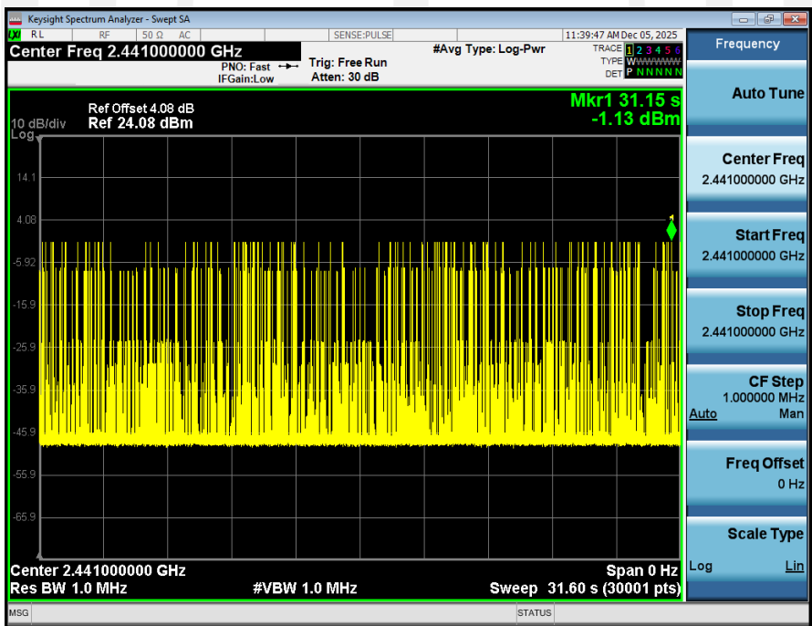
Dwell_Time_(Hopping)_NVNT_ANT1_2-DH5_2441_00_Accumulated
