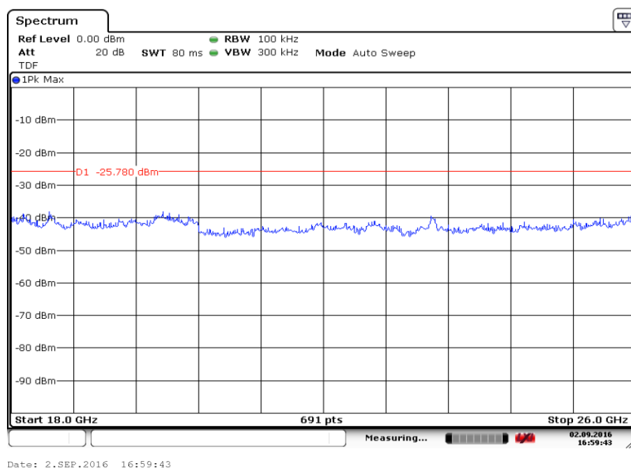
Fig.21 Conducted Spurious Emission (All channels, 18 GHz-26 GHz)
