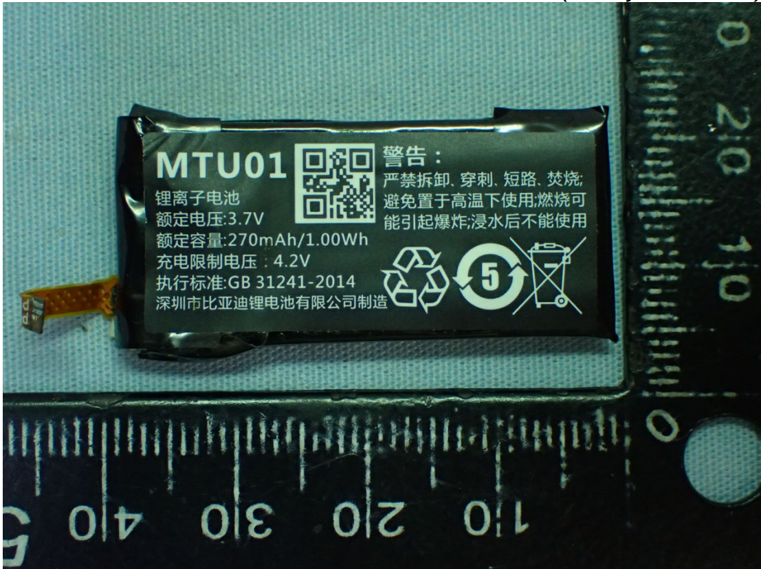
Figure 13 Internal View (Battery, Front View)
