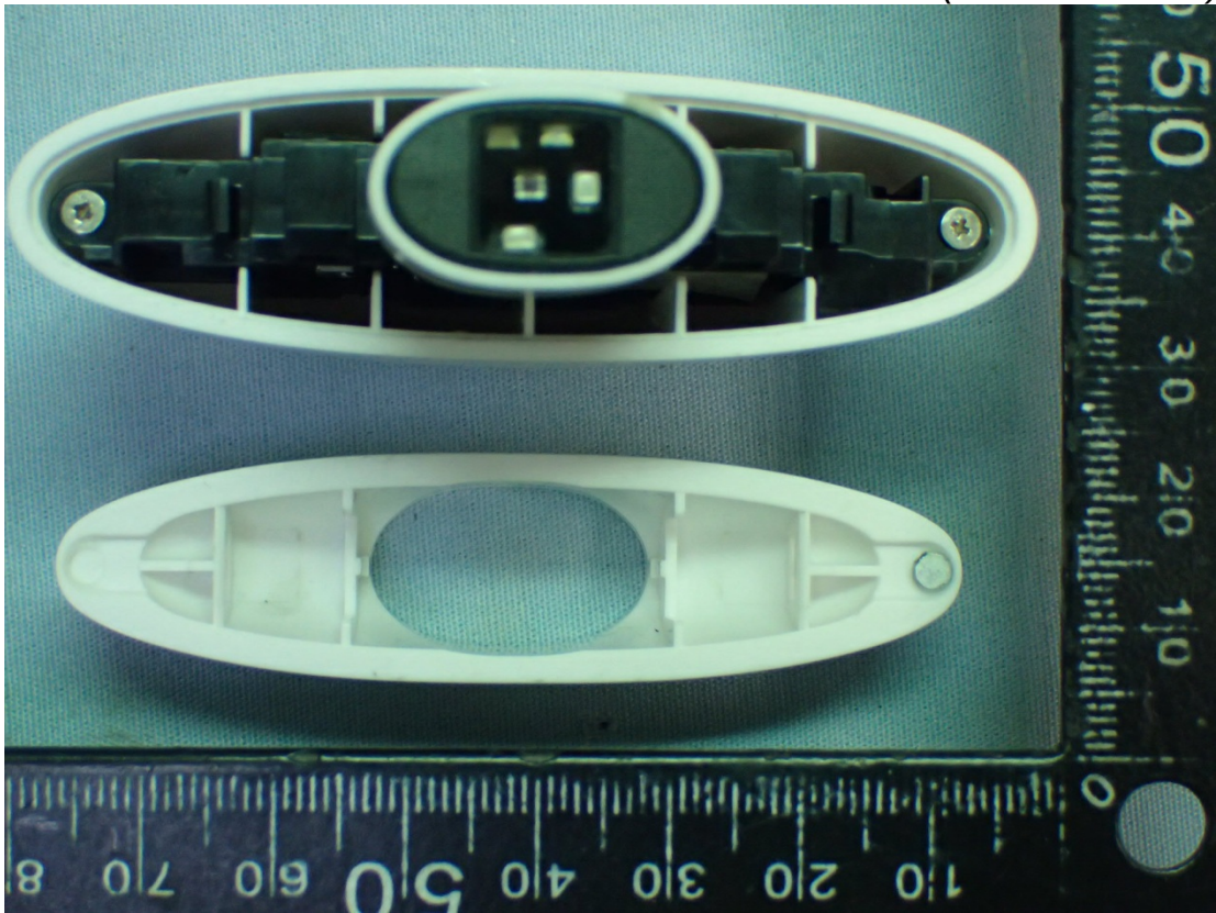
Figure 7 Internal View (Removed Cover)
