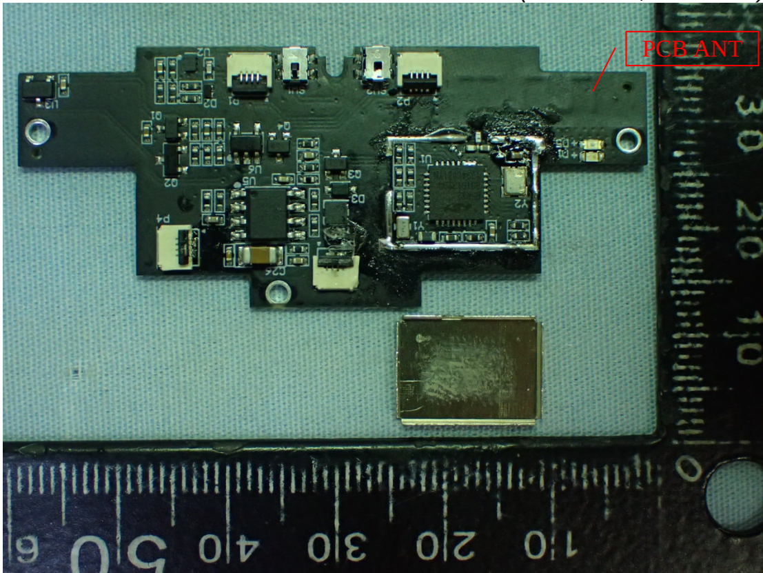
Figure 17 Internal View (Main Board, Front View)
