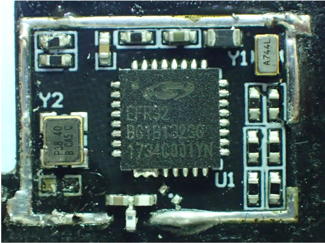
Figure 20 RF IC View
