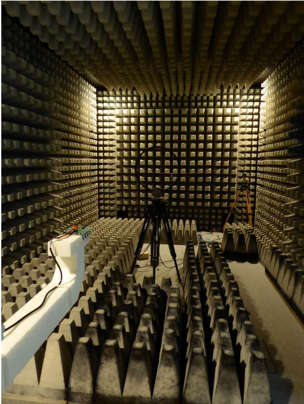
160903_02: Test setup - Radiated emission anechoic chamber
