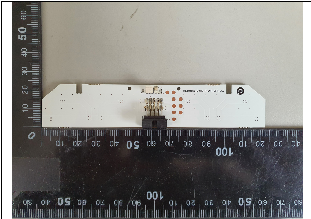
Front EXT Board Rear
